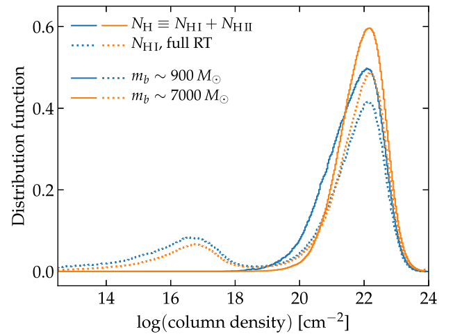
Figure A1. Column density distribution from stars \lesssim 10 Myr old out to the halo virial radius in galaxies around \log M_* \sim 8 . The solid and dashed lines show N_{\text{H}} and N_{\text{HI}} , respectively. The blue and orange lines show simulations at m_b \lesssim 900 M_\odot and \sim 7000 M_\odot resolution, respectively. At higher resolution, the distribution of N_{\text{H}} extends to lower column densities and a larger fraction of sightlines are optically thin, therefore resulting in systematically higher \langle f_{\text{esc}} \rangle at higher resolution.
