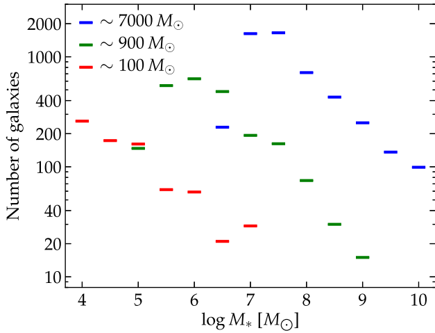
Figure 2. Number of galaxies for every 0.5 dex in stellar mass from M_* = 10^{3.75} – 10^{10.25} M_\odot in our simulation sample. We show the sample size for the three resolution levels but at all redshift.
