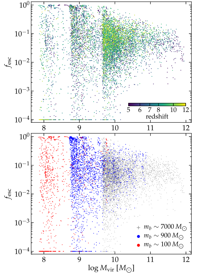
Figure 4. The f_{\text{esc}}-M_{\text{vir}} relation (using single-star and default dust model). Each point shows a halo snapshot in our simulated sample. In the top panel, the points are colour-coded by redshift. In the bottom panel, the colours represent the mass resolution of the simulation. The instantaneous f_{\text{esc}} has a large scatter (2–4 dex) at a given M_{\text{vir}} . Again, a high f_{\text{esc}} does not necessarily mean the galaxy is leaking a large number of ionizing photons, as the SFR may be low at these epochs.
