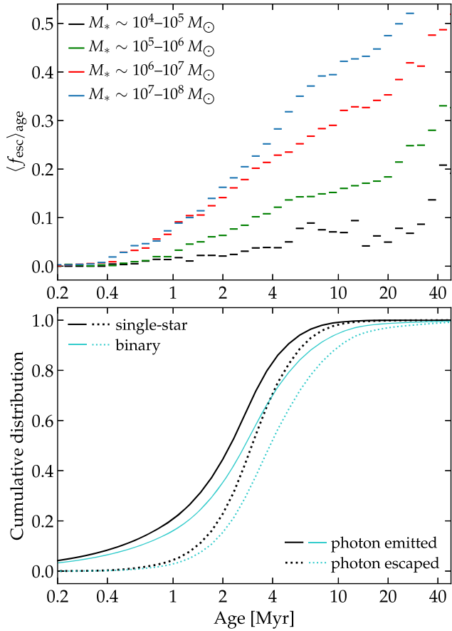
Figure 9. Top: The average escape fraction over individual stars in galaxies in four stellar mass bins for every 1/15 dex in logarithmic age. Only simulations at 900 M_\odot and better resolution are included. \langle f_{\text{esc}} \rangle_{\text{age}} increases with stellar age for galaxies of all masses. \langle f_{\text{esc}} \rangle_{\text{age}} increases with stellar mass at all ages, in line with the increase of sample average \langle f_{\text{esc}} \rangle with stellar mass in this mass range. Bottom: The cumulative distribution of ionizing photons emitted (solid) and escaped (dashed) as a function of stellar age. In single-star case (black), 50 per cent of the escaped ionizing photons come from stars 1–3 Myr old, while the rest 50 per cent from stars 3–10 Myr old. The binary models extend the distribution to slightly later times.
