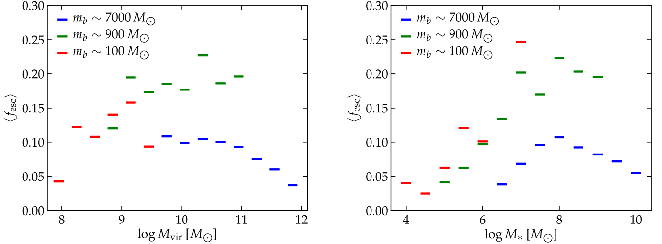
Figure 5. The sample average \langle f_{\text{esc}} \rangle as a function of M_{\text{vir}} (left-hand panel) and M_* (right-hand panel) (using single-star and default dust model). \langle f_{\text{esc}} \rangle is defined as the Q_{\text{ion}} -weighted instantaneous f_{\text{esc}} over all snapshots at all redshifts in a given halo/stellar mass bin. The blue, green, and red bars represent simulations at m_b \sim 7000 , 900 , and 100 M_{\odot} resolution. Our results do not fully converge with resolution. Simulations at m_b \sim 7000 M_{\odot} resolution tend to produce lower \langle f_{\text{esc}} \rangle than simulations at m_b \sim 900 M_{\odot} or better resolution. \langle f_{\text{esc}} \rangle increases with M_{\text{vir}} in \log M_{\text{vir}} \sim 8 – 9.5 , becomes nearly independent of M_{\text{vir}} in \log M_{\text{vir}} \sim 9.5 – 11 , and decreases with M_{\text{vir}} above \log M_{\text{vir}} \sim 11 . \langle f_{\text{esc}} \rangle increases with M_* up to \log M_* \sim 8 and decreases with M_* at higher masses. The decrease of f_{\text{esc}} at the high- and low-mass end is due to increasingly strong dust attenuation (cf. Fig. 6 and Section 3.2.2) and inefficient star formation and feedback (cf. Figs 9–11 and Section 4.4), respectively. It is worth noting that the compromise between these two effects results in the apparent independence of \langle f_{\text{esc}} \rangle on M_{\text{vir}} in \log M_{\text{vir}} \sim 9.5 – 11 .
