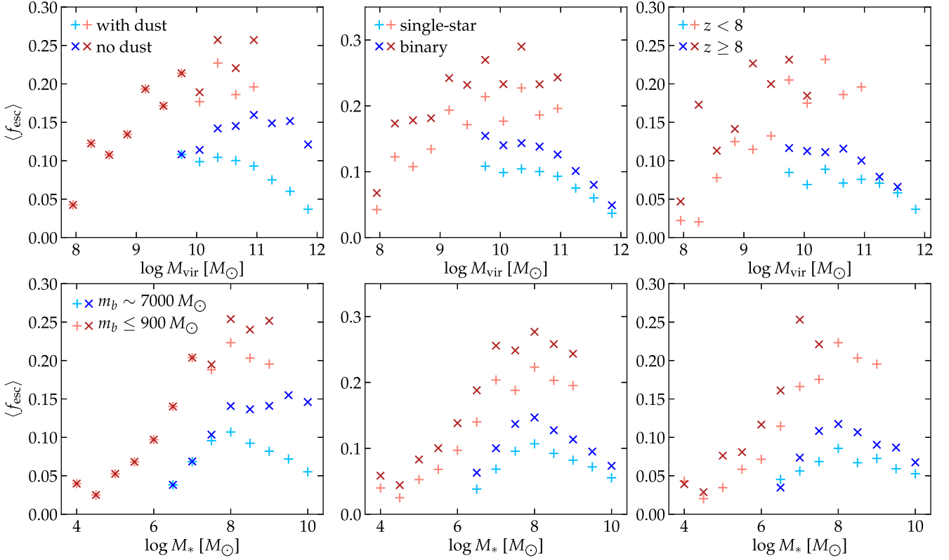
Figure 6. The \langle f_{\text{esc}} \rangle - M_{\text{vir}} (top) and \langle f_{\text{esc}} \rangle - M_{*} (bottom) relation, separated by simulations at 7000 M_{\odot} resolution (blue) and at 900 M_{\odot} resolution or better (red). Left-hand column: \langle f_{\text{esc}} \rangle with (light plus signs) and without (dark cross signs) dust attenuation. \langle f_{\text{esc}} \rangle increases with halo (stellar) mass up to \log M_{\text{vir}} \sim 11 ( \log M_{*} \sim 8 ) and becomes roughly constant at higher masses without dust attenuation, suggesting the decrease of \langle f_{\text{esc}} \rangle at the high-mass end in Fig. 5 is due to dust attenuation (Section 3.2.2). Middle column: \langle f_{\text{esc}} \rangle calculated using single-star (plus) and binary (cross) stellar population models. Binary models tend to boost \langle f_{\text{esc}} \rangle by \sim 25 – 35 per cent in most mass bins, as they predict more ionizing photons for a stellar population after 3 Myr and the extra photons have a higher possibility to escape (cf. Fig. 9 and Section 4.3). Binary stars increase the number of ionizing photons emitted by \sim 20 – 30 per cent, and thus the number of ionizing photons escaped by \sim 60 – 80 per cent (Section 3.2.3). Right-hand column: The dependence of \langle f_{\text{esc}} \rangle on redshift. The sample is divided into two redshift bins: z < 8 (plus) and z \geq 8 (cross). Galaxies at higher redshifts tend to have systematically higher \langle f_{\text{esc}} \rangle than galaxies at lower redshifts (Section 3.2.4).
