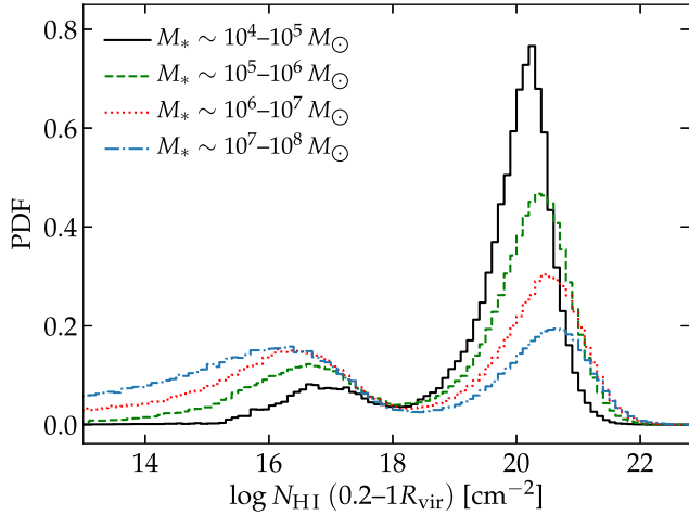
Figure 11. The distribution of N_{\text{HI}} integrated radially from 0.2 to 1R_{\text{vir}} in the halo of galaxies in four stellar mass bins. We include 1000 radial directions for each galaxy. All galaxies are equally weighted. The fraction of optically thin sightlines increases with stellar mass. The low-mass galaxies are nearly fully surrounded by optically thick gas in the halo.
