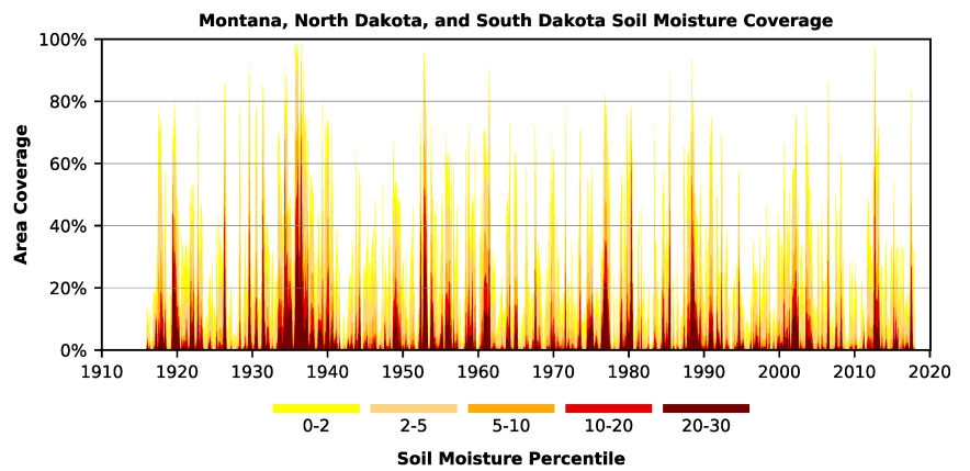
Fig. 3. Percentage of North Dakota, South Dakota, and Montana covered by soil moisture percentiles based on the UCLA Surface Water Monitor. This figure is adapted from Hoell et al. (2019a).
