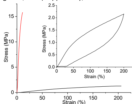
Figure 2. Stress-strain curves of plastic product from entry 8 of Table 1 (red) and elastic product from entry 9 of Table 1 (black). The inset is the stress-strain curve of a cyclic tensile test of the elastic sample. Toughness (area under the tensile curve) of the samples are 1.62 and 1.16 MJ/m 3 , respectively.
