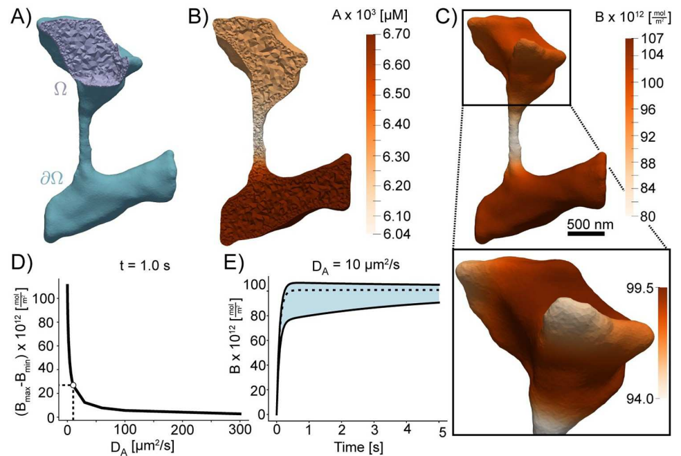
Fig 10. Simulations of coupled surface volume diffusion. A) Illustration of the domains for the volume and surface PDEs. B) and C) The concentrations of species A and B, respectively, at t = 1.0\text{s} when D_A is set to 10 \mu\text{m}^2/\text{s} . D) Difference between maximum and minimum values of B at t = 1.0\text{s} ; the point D_A = 10 \mu\text{m}^2/\text{s} corresponding to panels B) and C) is marked. E) the minimum, mean, and maximum of B over time when D_A = 10 \mu\text{m}^2/\text{s} ; a vertical bar is drawn at t = 1.0\text{s} . Scale bar: 500nm.
