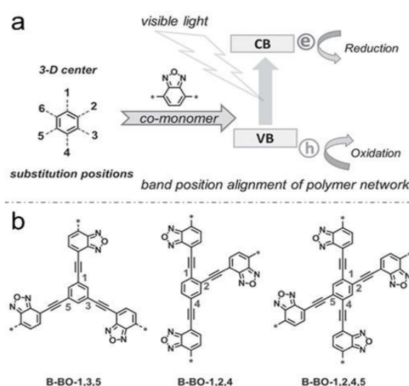
Fig. 12 (a) Geometry design principle of valence and conduction band position modification. (b) Synthesis of CMPs with the substitution
