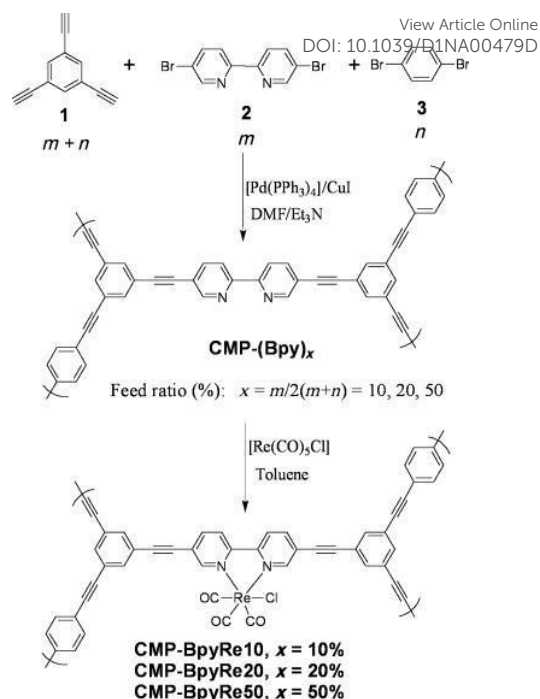
Fig. 6 Synthesis of metal-CMP via post-synthetic metalation. Adapted with permission. 114 Copyright 2010, John Wiley and Sons.
