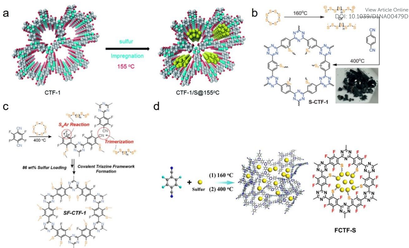
Fig. 16 (a) Synthesis of sulfur-containing CTF-1 by impregnation of molten sulfur. Reproduced with permission. 152 Copyright 2014, Royal Society of Chemistry. (b) Synthesis of S-CTF-1 from elemental sulfur in situ and (c) synthesis of SF-CTF-1 involving elemental sulfur-mediated nitrile trimerization along with the simultaneous covalent attachment of elemental sulfur via S N Ar chemistry. Reproduced with permission. 153,154 Copyright 2016 and 2017, John Wiley and Sons. (d) Synthesis of the FCTF-S composite by one-step sulfur-assisted cyclotrimerization of aromatic nitriles. Reproduced with permission. 155 Copyright 2017, American Chemical Society.
