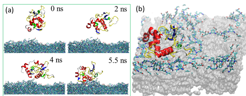
Figure 2. Lysozyme adsorption on the PA membrane: (a) lysozyme adsorption trajectory; (b) full adsorption of the lysozyme at 5.5 ns [top interfacial layer of membrane (top 0.4 \text{ nm} ) is rendered with a ball and stick model; the rest of the membrane is rendered with a gray colored ball model].
