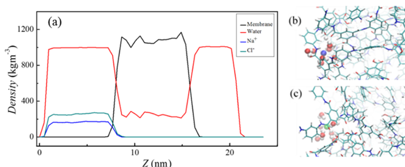
Figure 8. (a) Density distribution of the PA membrane, water, and ions (Na + and Cl - ); (b) snapshot of hydrated Na + ion on the PA membrane surface; and (c) snapshot of Cl - ions on the PA membrane surface. The configurations within the last nanosecond were used to compute the average density distribution at \Delta P = 5 MPa. It should be noted that the density is defined as the mass divided by the total volume at the Z position in the space. Note: the density was computed using the whole volume without taking into account the polymer exclusion volume.
