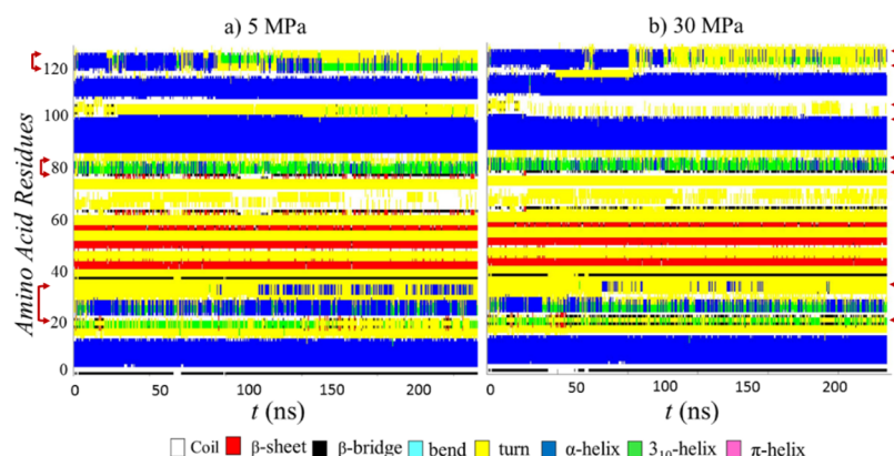
Figure 3. Time evolution of the secondary structure of an adsorbed lysozyme on the PA membrane surface for the case of 5 and 30 MPa pressure difference. Larger structural changes are denoted with red arrow marks.
