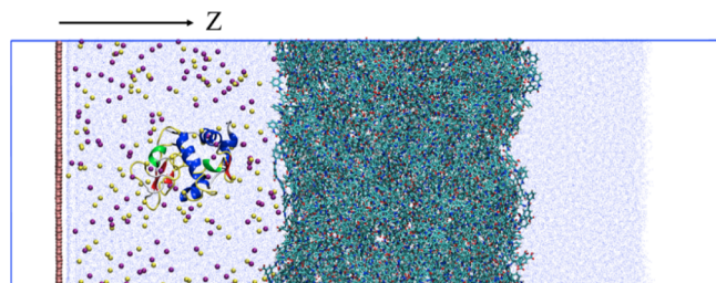
Figure 1. Initial configuration of NEMD of the PA membrane by pulling the graphene wall in the Z direction, which is normal to the graphene surface.
