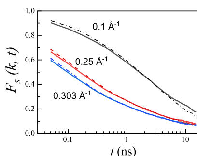
Figure 7. SISF F_s(\mathbf{k}, t) of oxygen atoms of water molecules inside the membrane at wavenumbers k = 0.1, 0.25 , and 0.303 Å −1 for the membrane at equilibrium conditions (straight lines) and the nonequilibrium with \Delta P = 0.5 MPa (dash-dot lines).
