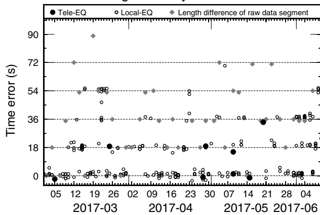
Figure 4. Time differences between the observed and theoretical arrivals of OBS PG01 station based on eight teleseismic earthquakes (black dots) and local earthquakes (open dots). Gray diamonds show the length differences of raw data segments relative to normal length. EQ, earthquake.
