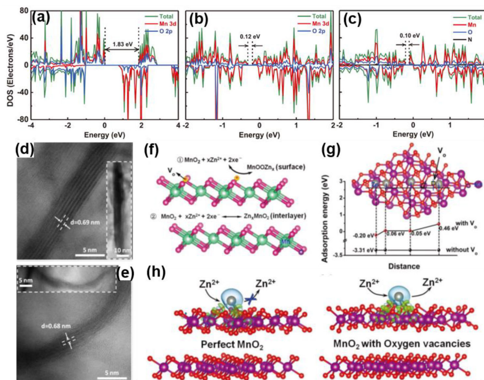
FIGURE 8 DOS of (A) MnO 2 , (B) MnO 2-x , and (C) N-MnO 2-x (reproduced with permission from ref. [101]; copyright 2019, Wiley-VCH). (D) Atomically resolved scanning transmission electron microscopy-annular bright-field (STEM-ABF) image of a C-MnO 2 nanosheet, with a larger view of the straight nanosheet in the inset. (E) Atomically resolved STEM-ABF image of one curved Od-MnO 2 nanosheet, with a larger view of the nanosheet in the inset. (F) Schematic illustration of oxygen-deficient \sigma -MnO 2 for Zn ion storage. (G) Calculated adsorption energies for Zn 2+ on the surfaces of pristine and oxygen-deficient \sigma -MnO 2 . Four possible sites for Zn adsorption are selected with a different distance from oxygen vacancy (VO). (h) Schematic illustration of Zn 2+ adsorption/desorption on pristine and oxygen-deficient MnO 2 (reproduced with permission from ref. [99]; copyright 2019, Wiley-VCH)
