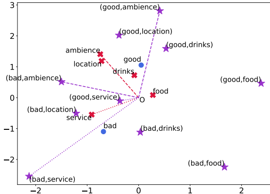
Figure 5: Visualization of joint topics (purple stars), aspect topics (red crosses) and sentiment topics (blue dots) in the embedding space.
