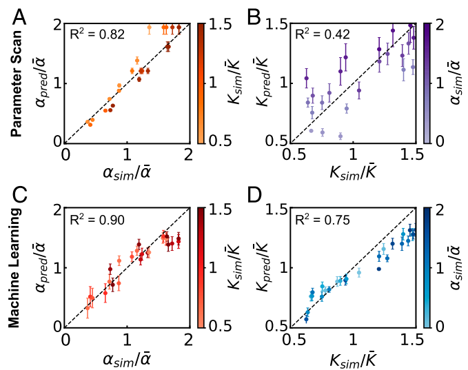
Fig. 2. Comparison of multiparameter estimation using neural networks and a high-throughput parameter scan. (A and B) Simultaneous estimation of \alpha and K using a high-throughput parameter scan ( SI Appendix , SI Text ). (C and D) Multiparameter estimation using our neural network. The network estimator outperforms the parameter scan approach for the predictions of both \alpha and K . Here \bar{\alpha} and \bar{K} are the mean values of \alpha and K from the training dataset. We quantify the performance for each parameter using the R^2 of the linear fit between the predictions and the ground truth (dashed line).
