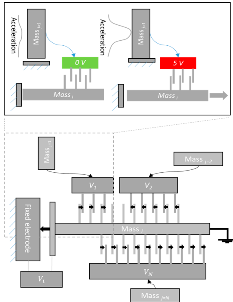
Figure 5. The finger arrays approach to realize electrostatic coupling between the MEMS CTRNs.
