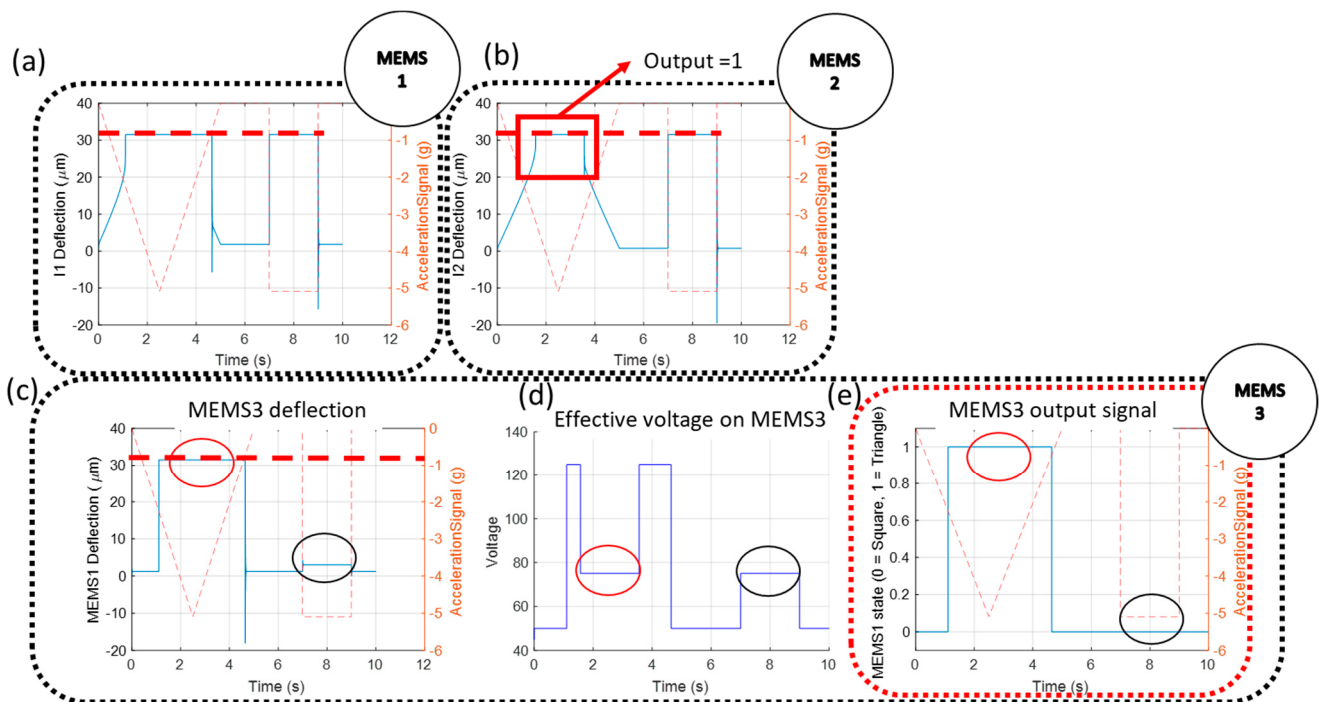
Figure 7. Classification test results showing the response of MEMS1 (a), MEMS2 (b) and MEMS3 (c). (d) The effective voltage acting on MEMS3 V_3(t) . (e) The state of MEMS3 when subject to a triangle or a square signal.
