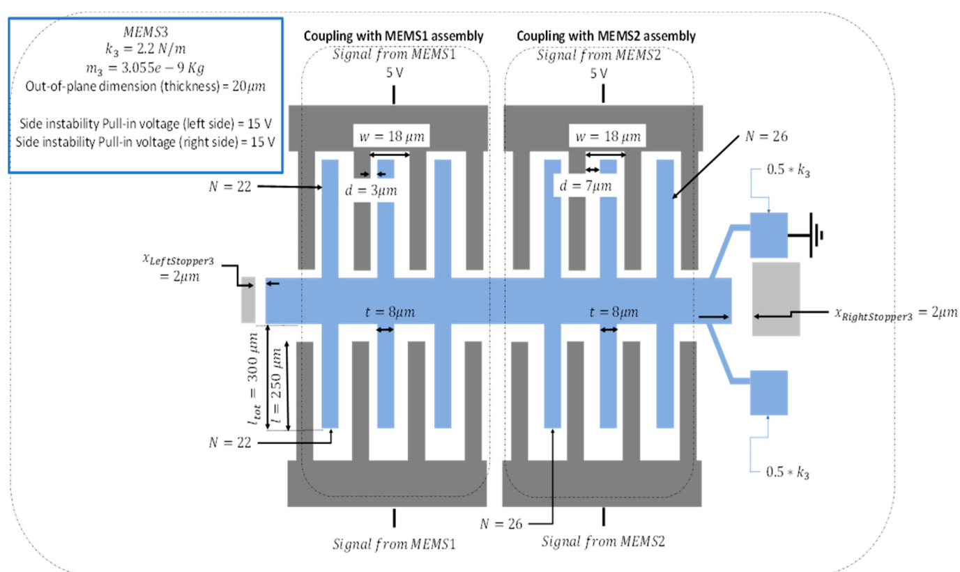
Figure A1. Design of the computing MMES device (labeled MEMS3 in Section 4), including information about the total stiffness of the MEMS device and the pull-in voltage.
