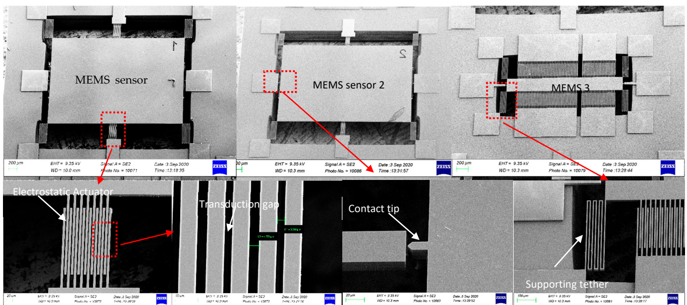
Figure 11. Scanning electron microscope (SEM) views of a fabricated MEMS CTRNN. This novel MEMS network can perform intelligent computing using only bias voltages.
