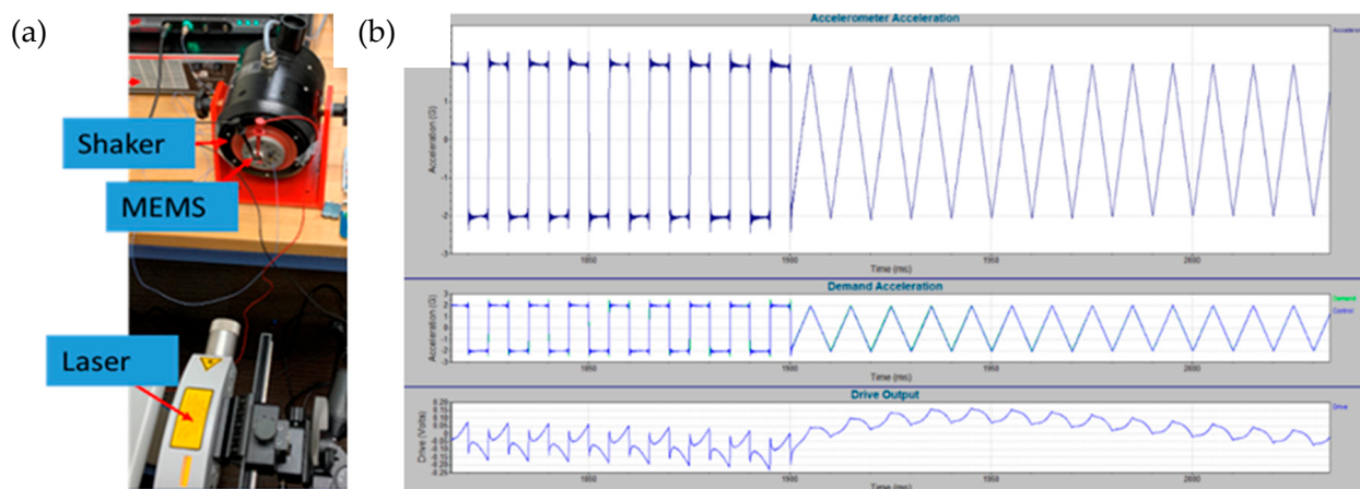
Figure 12. (a) The experimental set up to test the MEMS CTRNN, (b) samples of the triangle and square acceleration profiles generated by the mechanical shaker.
