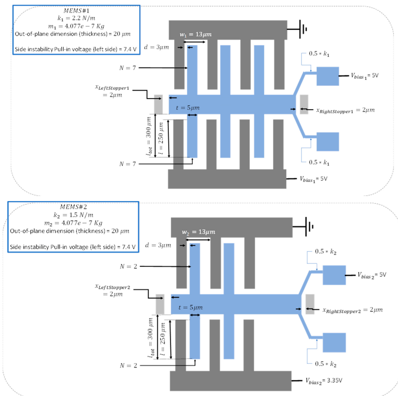
Figure A2. Design of the input layer MMES device (labeled MEMS1 and MEMS2 in Section 4), including information about the total stiffness of the MEMS devices and the pull-in voltages. Top figure: MEMS1, bottom figure: MEMS2.
