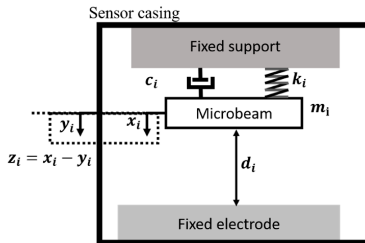
Figure 4. MEMS Schematic.
