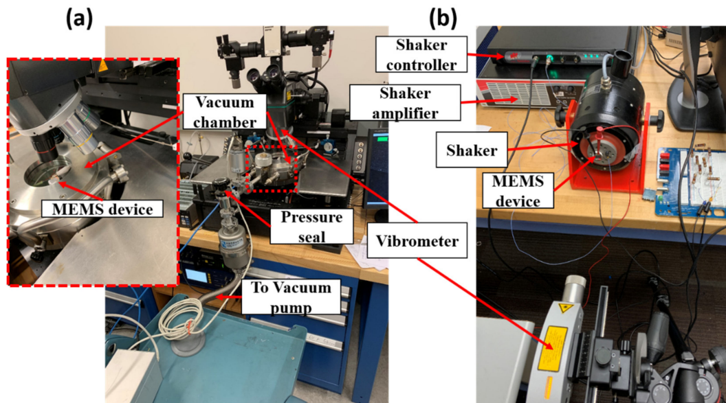
Figure 3. (a) Experimental setup for electrical waveform classification. The MEMS device is placed in a vacuum chamber to reduce pressure. The MEMS device serves as the reservoir in the RC system. The readout circuit is incorporated using an external data digital processor. The deflection of the MEMS device is attained by integrating the velocity signal from the laser vibrometer. (b) Experimental setup for acceleration waveform classification. The MEMS device is fixed on a shaker. The MEMS response is measured as the difference between the microbeam and ceramic base deflections. The shaker is controlled through a dedicated adaptive controller.
