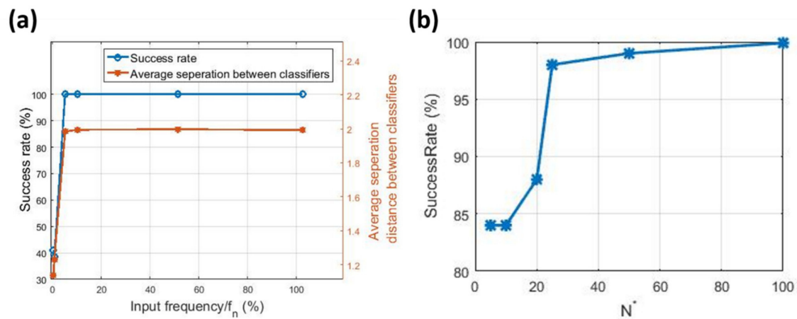
Figure 4. (a) Classifier accuracy as a function of the input frequency. At low input frequencies, the classifier fails to classify the input signal. However, as the frequency increases, the reservoir prediction accuracy increases to >99%. (b) MEMS RC classification performance at f/f_n = 20\% when different N are considered.
