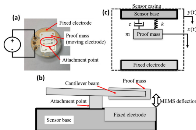
Figure 2. Microelectromechanical systems (MEMS) device schematics. (a) MEMS accelerometer used in this study. (b) Schematics of the MEMS side view showing the fixture the electrostatic gap. (c) Single-degree of freedom model of the MEMS accelerometer. Here, c = 2\zeta m_{eff}(2\pi f_n) is the damping constant and k = (2\pi f_n)^2 m_{eff} is the linear stiffness of the MEMS device.
