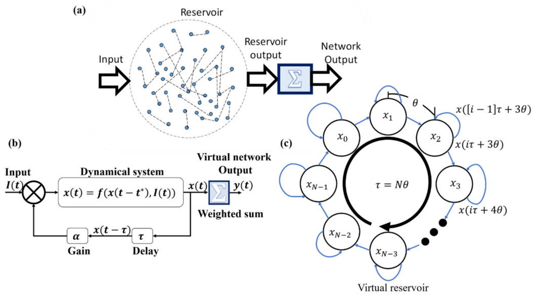
Figure 1. Reservoir computing (RC) schemes. (a) Classical RC utilizes a large network of randomly connected neurons. The output of the reservoir is a simple weighted sum of the neuronal response. (b) Delay-based RC utilizes the properties of dynamical systems and delayed feedback. (c) The virtual reservoir produced from delayed feedback and system dynamics.
