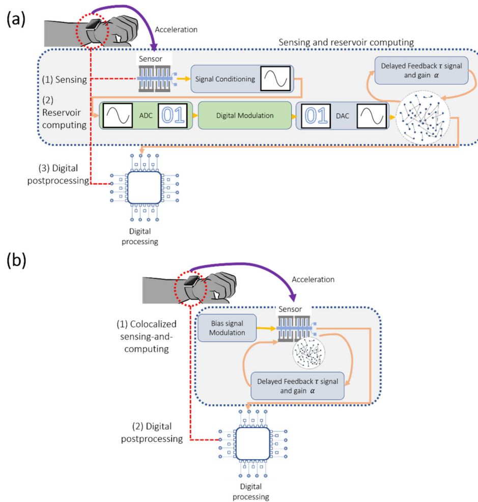
Figure 7. Illustration demonstrating the size reduction of the RC scheme with the use of sensors for colocalized sensing-and-computing. In this figure, digital components are represented by green blocks. Analog components are represented by grey components. (a) Delay RC scheme with separated sensing and computing. (b) Delay RC scheme with colocalized sensing and computing.
