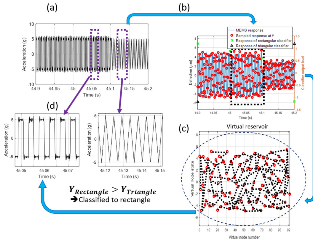
Figure 6. MEMS sense-and-compute scheme: (a) a sample of the acceleration signal generated by the shaker. (b) The response of the MEMS device and virtual node extraction. (c) Visualization of the virtual reservoir within the network. The response of the virtual nodes shown in this figure is used to compute the reservoir output after all the virtual nodes are updated. (d) Classification process based on the RC output.
