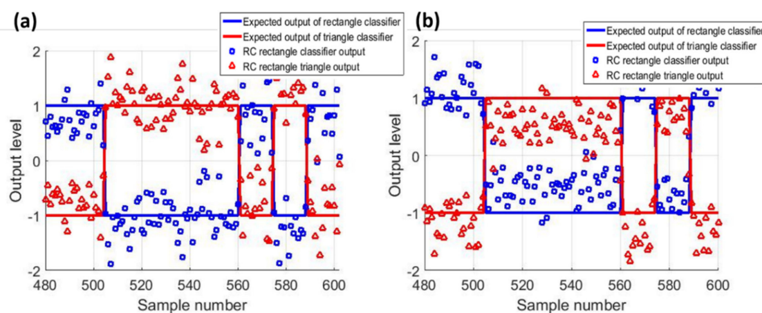
Figure 5. Experimental classification of low-frequency signal using the MEMS RC (a) under parameter (pressure) drift (b) and colored noise. The real-time results of the RC show success rates of 99.8% and 99.66%, respectively.
