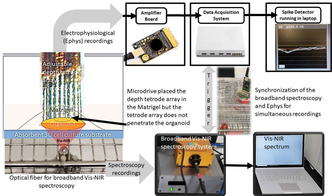
Figure 1. Experimental setup combining broadband vis/near-infrared spectroscopy and electrophysiology. The setup consists of a 32-channel tetraode microdrive integrated with the Intan RHD2132 amplifier (Intan Technologies, USA) and Open Ephys data acquisition system. Intan RHD2132 amplifier (Intan Technologies, USA) supports sampling 32 amplifier channels at 30 kSamples/s each, and provide fully integrated electrophysiology amplifier array with on-chip 16-bit analog-to-digital converter (ADC). We used the Open Ephys GUI and Spike Detector plugin for online monitoring of the data fidelity across the channels as well as for data recording in a laptop computer. Broadband Vis-NIR spectroscopy system consisted of the SILVER-Nova spectrometer (Stellarnet, USA) over the 190–1110 nm wavelength range with 200 \mu\text{m} slit for high sensitivity, SL1 high stability Tungsten Halogen light (350–2500 nm) source (Stellarnet, USA), and R600-8-VisNIR Reflectance Probe (Stellarnet, USA) for VIS-NIR spectroscopy with seven optical fibers bundled around one 600 \mu\text{m} fiber. We used the SpectraWiz spectrometer software (Stellarnet, USA) for recording the Broadband Vis-NIR spectroscopy data on a laptop computer.
