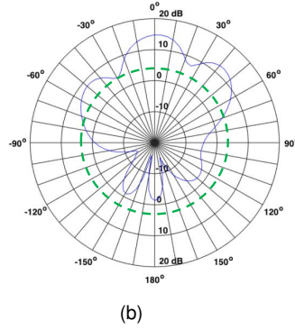
Fig. 3: (a) Experimental setup showing X60 platform with NI mm-Wave transceivers and SiBeam’s phased array antenna. (b) Irregular azimuth beam pattern and its average directivity (green) (c) Experimental setup showing WARP-60 platform with 60 GHz signal and control flow.
