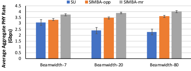
Fig. 7: Average of the aggregate rate for all the users in the setup.
