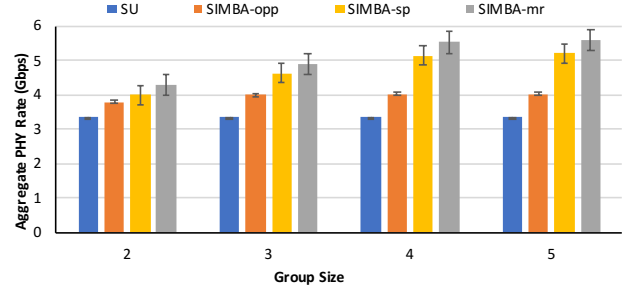
Fig. 9: Achievable aggregate rate vs. number of simultaneous users
