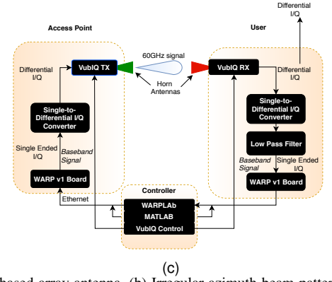
Fig. 3: (a) Experimental setup showing X60 platform with NI mm-Wave transceivers and SiBeam’s phased array antenna. (b) Irregular azimuth beam pattern and its average directivity (green) (c) Experimental setup showing WARP-60 platform with 60 GHz signal and control flow.
