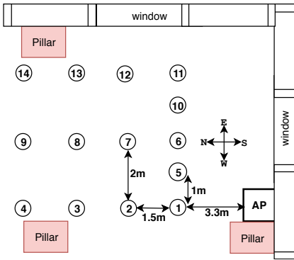
Fig. 8: Experimental layout consisting of AP and 14 users (shown in circles)
