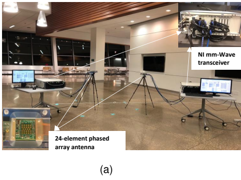
Fig. 3: (a) Experimental setup showing X60 platform with NI mm-Wave transceivers and SiBeam’s phased array antenna. (b) Irregular azimuth beam pattern and its average directivity (green) (c) Experimental setup showing WARP-60 platform with 60 GHz signal and control flow.
