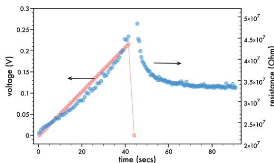
Fig. 9 Decay response of a ITO/pC6DTP ox /Al memristor after the cessation of a linear-increasing voltage pulse train.
