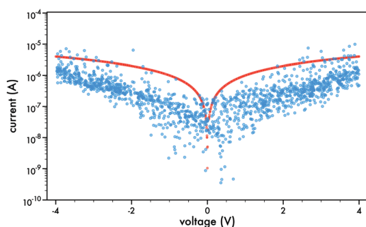
Fig. 5 Conductance of pC6DTP ox device (blue) with random excitatory voltage pulses. Device was ITO/pC6DTP ox /Al and was measured at 23 °C. Stochastic voltage–current relationship of 1 MΩ standard resistor (red) is also presented.
