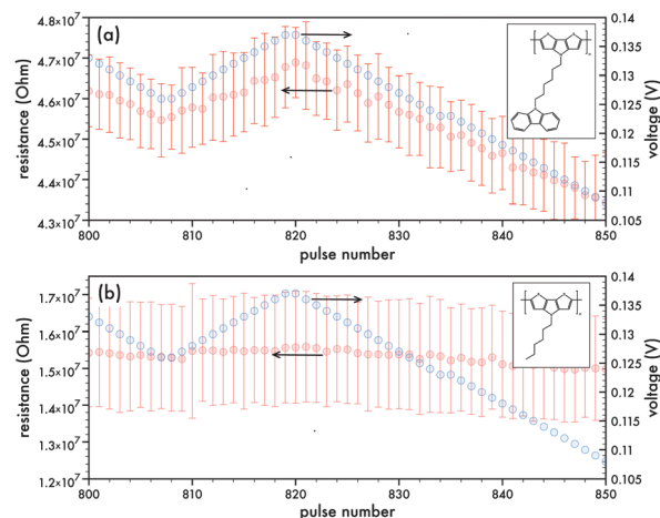
Fig. 11 Average resistance response (red) with an applied potential profile (blue) with 1 mV increment of (a) pC6DTP ox and (b) p6DTP ox device. Device was subjected to same voltage profile 10 times and error bars represent standard deviation from mean. Inset presents structure of polymer repeat unit.
