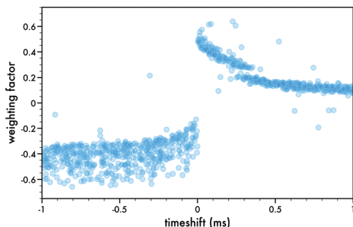
Fig. 7 Spike-timing-dependent-plasticity (STDP) of ITO/pC6DTP ox /Al memristor.
