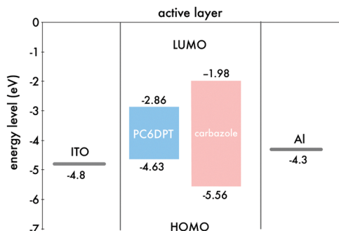
Fig. 4 Electronic characteristics of neutral pC6DTP measured by UV-vis spectroscopy and cyclovoltammetry; all energies expressed in eV and are relative to the vacuum level. LUMO values are based on the difference of the measured oxidation potential (HOMO) and the energy at the experimentally observed electronic absorption band edge. The experimentally derived HOMO/LUMO energy values of 9H-carbazole (carbazole) are presented for reference purposes.
