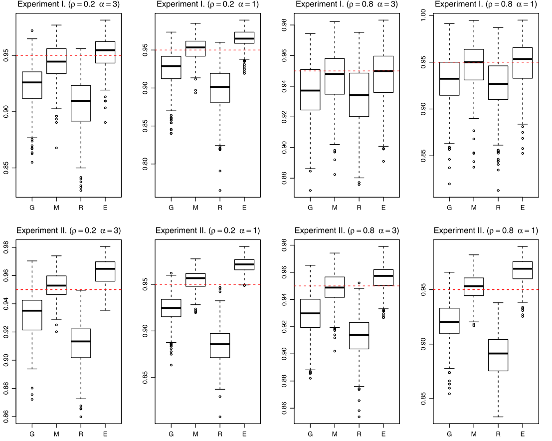
FIG. 1. Simulated relative frequency of the simultaneous coverage of 500 95% simultaneous confidence intervals for each bootstrap scheme: G, M and R, respectively, represent the Gaussian, Mammen and Rademacher wild bootstrap, while E represents Efron's empirical bootstrap.
