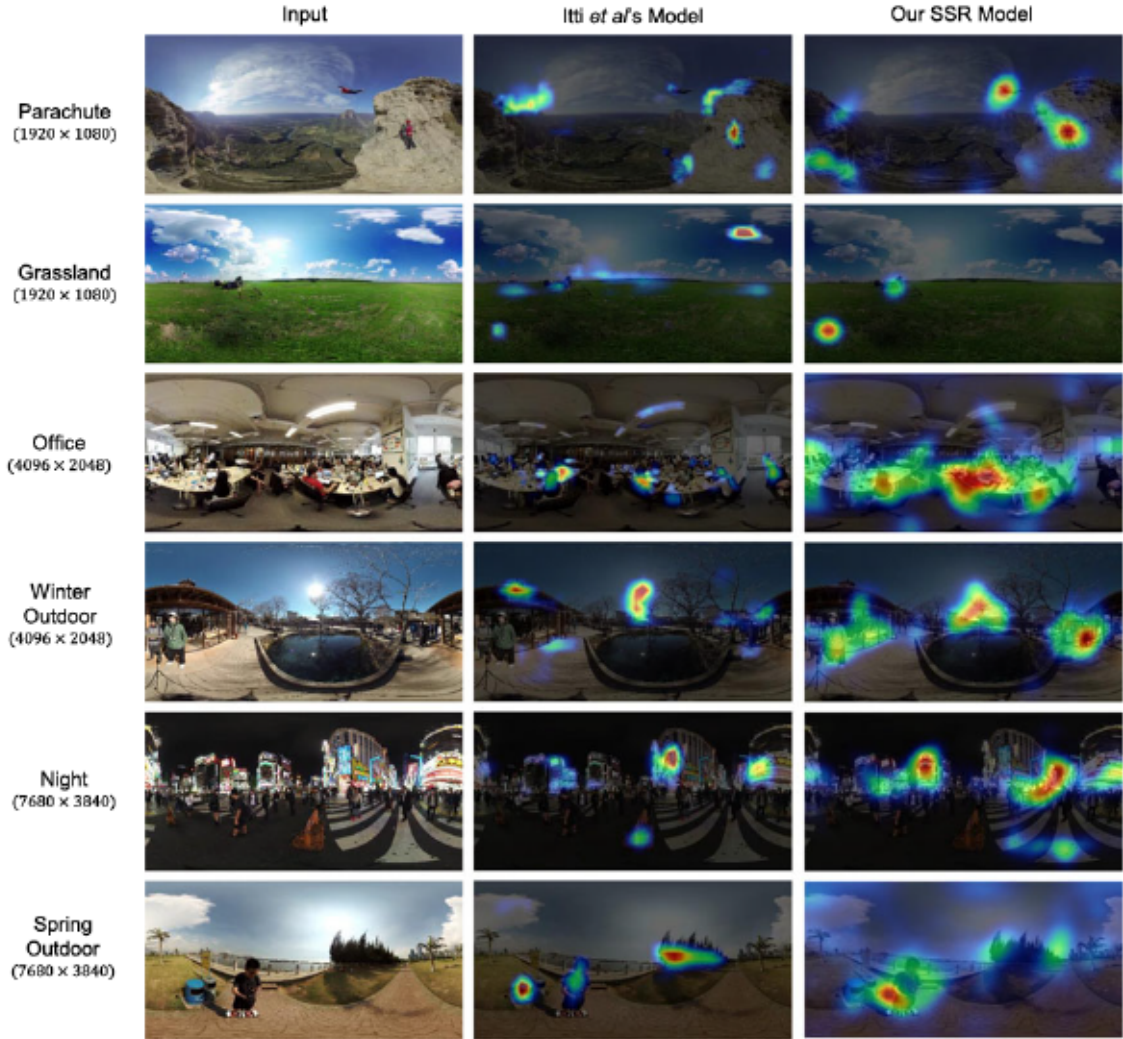
FIGURE 5. Visual comparison between the Itti et al. model and our SSR model. Note that while the results are visually similar, our SSR model is 5\times to 13\times faster than the Itti et al. model.
