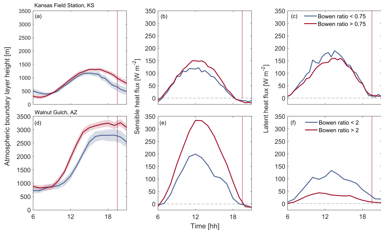
Fig. 5. (a) Mean diurnal development of the atmospheric boundary layer height (ABLH) in July 2017 at the Kansas Field Station flux tower site (US-KFS) on days with low Bowen ratio ( < 0.75 ) and high Bowen ratio ( > 0.75 ) and mean diurnal variation of (b) sensible and (c) latent heat fluxes on days with low and high Bowen ratio. (d) Mean diurnal development of ABLH between July and September 2019 at the Walnut Gulch flux tower site (US-Wkg/Whs) on days with low Bowen ratio ( < 2 ) and high Bowen ratio ( > 2 ) and mean diurnal variation of (e) sensible and (f) latent heat fluxes on days with low and high Bowen ratio at the same site. Vertical red dotted lines indicate the approximate timing of sunset. Atmospheric boundary layer heights were derived from aerosol backscatter profiles measured by ceilometers. Note that the detected early morning ABLH might be the top of the residual layer.
