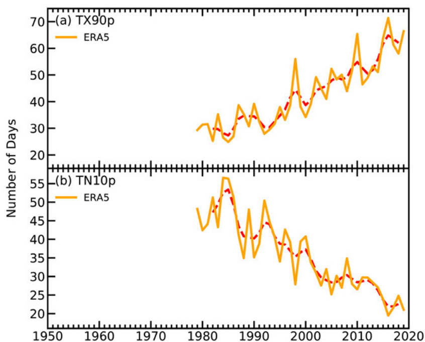
Fig. 2.5. Time series of (a) TX90p (warm days) and (b) TN10p (cool nights). The red dashed line shows a binomial smoothed variation. (Source: ERA5.)
