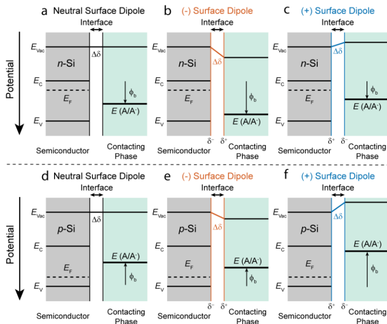
Figure 1. Diagram illustrating the shift in the relative positions of the bands for (a, b, c) n-type and (d, e, f) p-type semiconductor, and the contacting electrolyte layer induced by (a, d) no, (b, e) negative, and (c, f) positive dipole layers. In this figure, E_C , E_V , E_F , and E_{Vac} represent the potentials of the conduction-band-edge minimum, valence-band-edge maximum, Fermi-level and the vacuum level, respectively. The shift in the vacuum level caused by the electric field within the dipole layer is represented as \Delta\delta . The barrier height, \phi_b , limits the attainable photovoltage.
