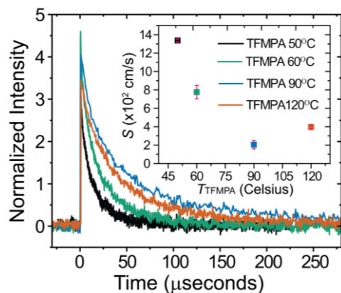
Figure 4. Time-resolved microwave conductivity measurements for mixed TFMPA/methyl-terminated silicon surfaces prepared by nucleophilic addition of TFMPA at 50 (black), 60 (green), 90 (blue) and 120 (red) ^\circ\text{C} . Inset figure is a summary of the average surface recombination velocity ( S ) as a function of the TFMPA addition temperature ( T_{\text{TFMPA}} ), averaged over six samples.
