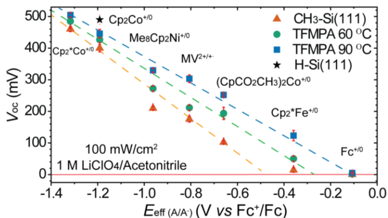
Figure 7. Open-circuit voltage ( V_{oc} ) of mixed TFMPA/methyl-terminated p-Si(111) electrodes submerged in acetonitrile electrolytes containing 1.0 \text{ M LiClO}_4 and under 100 \text{ mW cm}^{-2} (1 Sun) illumination. V_{oc} values are shown as a function of the effective solution potential ( E_{eff} ) for TFMPA addition temperatures of 60^\circ\text{C} (green circles) and 90^\circ\text{C} (blue squares), in comparison to a methyl-terminated p-Si(111) (red triangles). Each V_{oc} data point is the averaged result from 2–3 electrodes constructed from four reaction batches. The V_{oc} for hydrogen-terminated p-Si(111) (black star) using cobaltocene ^{+/0} as the redox couple has been included as an additional control.
