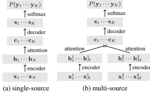
Figure 2: Simple visualization of the transformer model with a single- and multisource architecture. In the standard single-source model, the decoder attends to a single encoder’s states. In our multi-source setup, we have two input sequences encoded by two different encoders, and attention mechanisms provide two context to the decoder. Note that for clarity’s sake there are dependencies not shown.
