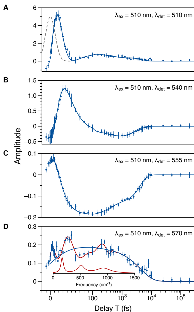
Figure 5. Amplitude transients after optical excitation of the per2,3 excitons in wtPCP-Chl a (A–D) The amplitude detected at (A) 510 nm, (B) 540 nm, (C) 555 nm, and (D) 570 nm in the 2DES spectrum (Figure 2) is superimposed in each panel with that obtained from the global model (smooth curves) as a function of T , which is plotted against a semilogarithmic axis split at 100 fs. The bars on each plotted data point report 95% confidence intervals for the amplitudes. (A) includes a dashed, 21-fs Gaussian showing the instrument-response function used in the global model, which is convoluted with the responses from the spectrokinetic species. In (D), the amplitude is plotted superimposed with a red curve showing a fit of the residual (signal – global model) to a rising, sum of damped cosinusoids function. The model parameters are listed in Table S5. The inset shows the frequency spectrum corresponding to the amplitude of the modulation components.
