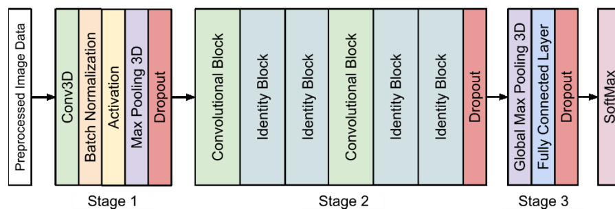
Figure 5. The architecture of the 3D CNN model used in this study. Details of the convolutional block and the identity block are shown in Figure 6.
