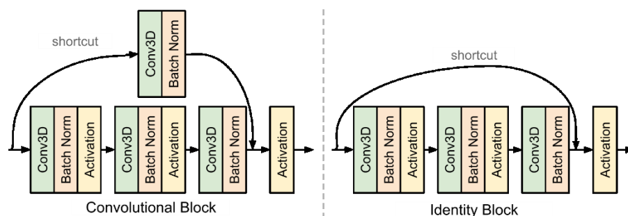
Figure 6. Details of the convolutional block and the identity block.
