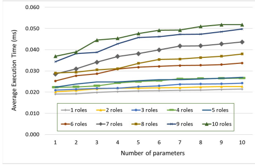
Fig. 5. Average execution time required to finish the tested operations.
