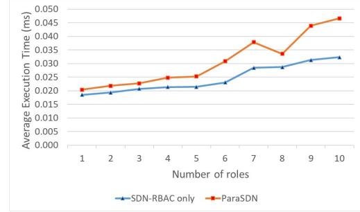
Fig. 6. Overhead imposed by parameters in ParaSDN compared to SDN-RBAC system.
