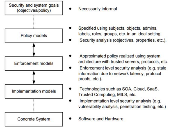
Fig. 2. The PEI Framework [7]
