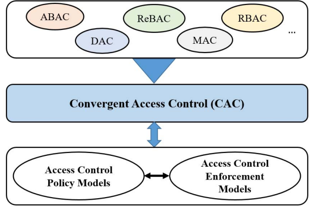
Fig. 5. The Convergent Access Control (CAC) Framework
