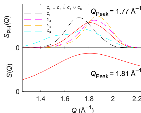
Fig. 5. Deconvolution of the FSDP. Comparison between the S_{\text{PH}}(Q) function calculated from Eq. 2 for all characteristic regions as well as their union and the structure factor [S(Q)] , both shown for the 20\text{Na}_2\text{O}-80\text{SiO}_2 glass. Note that we exclude C_T from this analysis.
