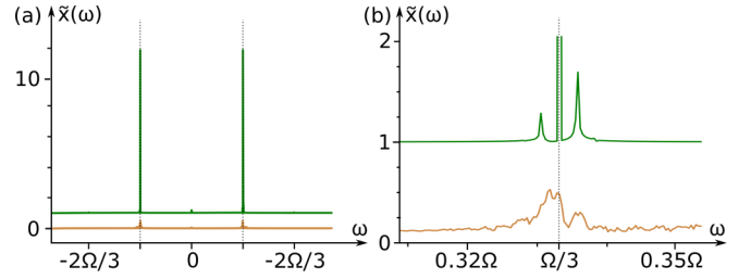
FIG. 3. Observable signatures of quantum frequency locking. (a) Frequency spectrum of the cavity field \langle \hat{x}(t) \rangle for the system when initialized within (green) and outside (orange) the frequency-locking regime, respectively. See main text for parameters and further details. Note that the green curve is vertically offset by 1. (b) Zoom-in of (a), in the vicinity of \omega = \Omega/3 (indicated by vertical dashed line).
