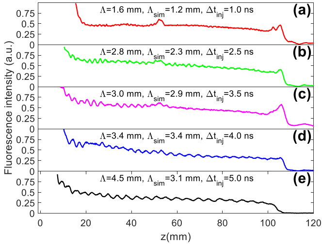
FIG. 7. Full length hydrogen plasma fluorescence (recombination) image lineouts of self-waveguiding (of \lambda = 800 nm, w_0 = 25 \mu m, 40 fs, 88-mJ pulses) in a 10-cm-long index structure generated in an elongated supersonic hydrogen jet by a 100-mJ J_0 pulse. Here the injection delay \Delta t_{inj} is varied from 1 to 5 ns, slightly changing the self-generated plasma waveguide [as seen in Fig. 3(d)] and its quasibound modes and wave numbers \beta_{0,0} and \beta_{1,0} , leading to a variation in the mode beating period \Lambda_{sim} = (\Delta\beta)^{-1} , where \Delta\beta = \beta_{0,0} - \beta_{1,0} . The simulated period \Lambda_{sim} and measured profile-average period \Lambda are in reasonable agreement. The bump at z \sim 50 mm is from light scattering from an optical support post in the experimental chamber.
