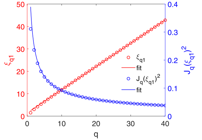
FIG. 11. Computation of \xi_{q1} and J_q^2(\xi_{q1}) vs q (red circles and blue circles). Fits are overlaid: (\xi_{q1})_{fit} = 1.03q + 1.44 and [J_q^2(\xi_{q1})]_{fit} = 0.39q^{-0.63} .
