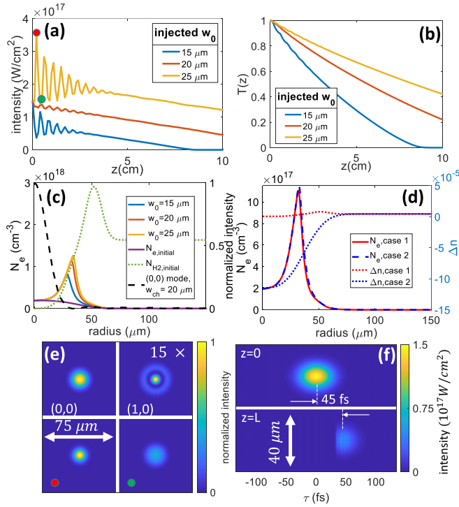
FIG. 5. Simulations of self-waveguiding. Peak input intensity at z = 0 is I_0 = 1.5 \times 10^{17} W/cm 2 . The panel descriptions are the same as in Fig. 4, except that in (e), the (1,0) mode is shown scaled in intensity by 15\times .
