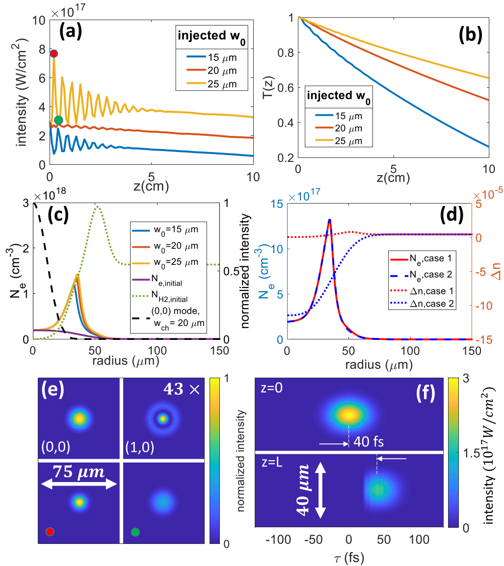
FIG. 4. Simulations of self-waveguiding. Peak input intensity at z = 0 is I_0 = 3 \times 10^{17} \text{ W}/\text{cm}^2 . (a) Peak laser intensity I(r = 0, z, \tau_{\text{peak}}) vs z for various injection pulse waists w_0 . (b) z -dependent transmission efficiency, T(z) = \varepsilon_i^{-1} \int d\tau d^2\mathbf{r}_\perp I(\mathbf{r}_\perp, z, \tau) , for the three input modes of (a), with variables defined in the text. (c) Similar N_e(r) profiles generated by varying w_0 mode injection into the initial index profile shown (characterized by N_{e, \text{initial}} and N_{H2, \text{initial}} ). The dashed black curve is the computed (see Appendix A and Ref. [22]), lowest-order quasibound mode of the generated plasma waveguide. (d) Demonstration that a range of possible initial refractive index structures (plotted as refractive index difference \Delta n = n - 1 ) can support self-waveguiding, with almost identical plasma waveguides generated. The main feature necessary for self-waveguiding is an on-axis neutral gas density depression. (e) Top two panels: (0,0) and (1,0) quasibound intensity modes of plasma waveguide in (b). The (1,0) mode is shown scaled in intensity by 43. Bottom two panels: propagating mode at z locations of intensity maximum and minimum [green and red dots in (a)]. (f) Pulse intensity envelopes in (r, \tau) at the entrance ( z = 0 , top panel) and exit ( z = L = 10 cm, bottom panel) of the index structure. The plots show pulse head erosion and group velocity delay in the self-generated waveguide. The pulse propagates right to left.
