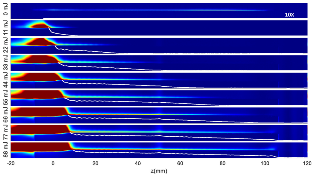
FIG. 6. Full length hydrogen plasma fluorescence (recombination) images of self-waveguiding of \lambda = 800 -nm, 40-fs pulses of increasing energy in a 10-cm-long index structure generated in an elongated supersonic hydrogen jet by a 100-mJ J_0 pulse. \Delta t_{\text{injection}} = 2.5 ns into the profiles of Fig. 3(a). The pulse propagates left to right. Below each image is a central lineout (white curves). The decreasing fluorescence with z indicates pulse head erosion of the self-waveguiding pulse. The bump at z \sim 50 mm is from light scattering from an optical support post in the experimental chamber. The saturated (brown) image at the jet entrance is from the injected laser pulse overfilling the initial index structure. The slight bump at the channel exit is from ionization of neutrals by the exiting pulse. The top panel shows fluorescence induced by the J_0 pulse alone.
