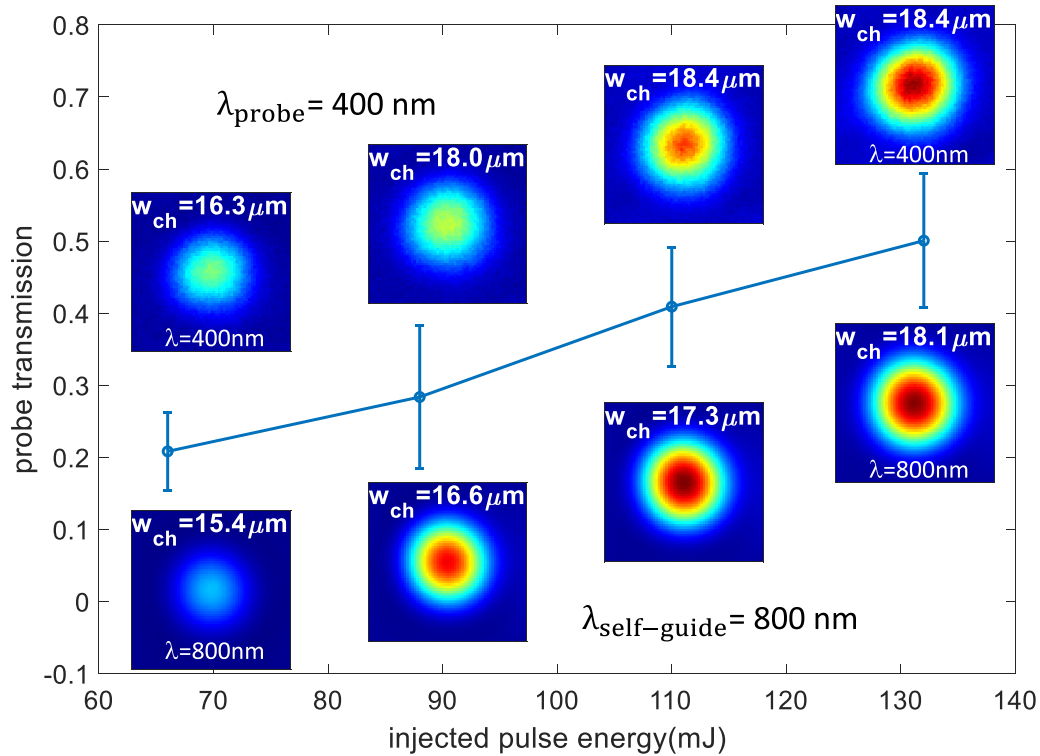
FIG. 9. Pump-probe experiment, where the pump is the self-waveguiding pulse ( \lambda = 800 \text{ nm} ) injected at \Delta t_{\text{inj}} = 2.5 \text{ ns} after the 100-mJ J_0 pulse, followed at 5 ps delay by a probe pulse ( \lambda = 400 \text{ nm} ). The corresponding initial index structure is plotted in Fig. 2(a), and its generated waveguide is shown in Fig. 3(a). The self-waveguided \lambda = 800\text{-nm} exit modes are shown below the curve, with the corresponding \lambda = 400\text{-nm} probe exit modes shown above the curve. The mode invariance ( w_{\text{ch}} = 16\text{--}18 \mu\text{m} ) illustrates that (i) the resulting plasma waveguide structure is nearly independent of the energy of the self-waveguiding pulse and (ii) the plasma waveguide mode structure is wavelength independent.
