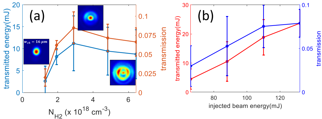
FIG. 8. (a) Plot showing hydrogen density threshold for self-waveguiding (injection pulse energy 88 mJ, \Delta t_{inj} = 2.5 ns). As density increases, both (0,0) and (1,0) modes are seen at the channel exit, with the contribution of the (1,0) mode increasing. The slightly reduced transmission at higher density may be from leakage of the (1,0) mode. (b) Injected pulse transmission vs energy (for \Delta t_{inj} = 2.5 ns and N_{H_2} = 3 \times 10^{18} cm ^{-3} ), where the low end of the energy axis is the minimum needed for burn-through of the 10-cm-long structure. Peak self-waveguided intensity exiting the guide is 1.5 \times 10^{17} W/cm ^2 .
