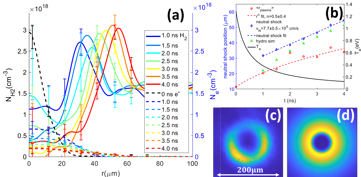
FIG. 2. (a) Plasma and neutral gas-density profile evolution measured by two-color transverse interferometry. (b) J_0 pulse-induced rms plasma column radius \langle r_{\text{plasma}} \rangle and neutral shock position vs time. The plasma temperature is computed from the plasma expansion (see text). The neutral shock speed v_N \sim 7.7 \times 10^5 cm/s, calculated from the plotted points, indicates a gas temperature \sim 0.4 eV. Green triangles: neutral shock position vs time from hydrodynamic simulation. (c) Ring mode image of \lambda = 400 -nm probe pulse trapped and guided in neutral shock cylindrical annulus. Hydrogen backfill, 50 torr. (d) Beam propagation method (BPM) simulation [18] using conditions of (c). Error bars, here and in subsequent plots, are from phase error propagation in Abel inversion (see Appendix C).
