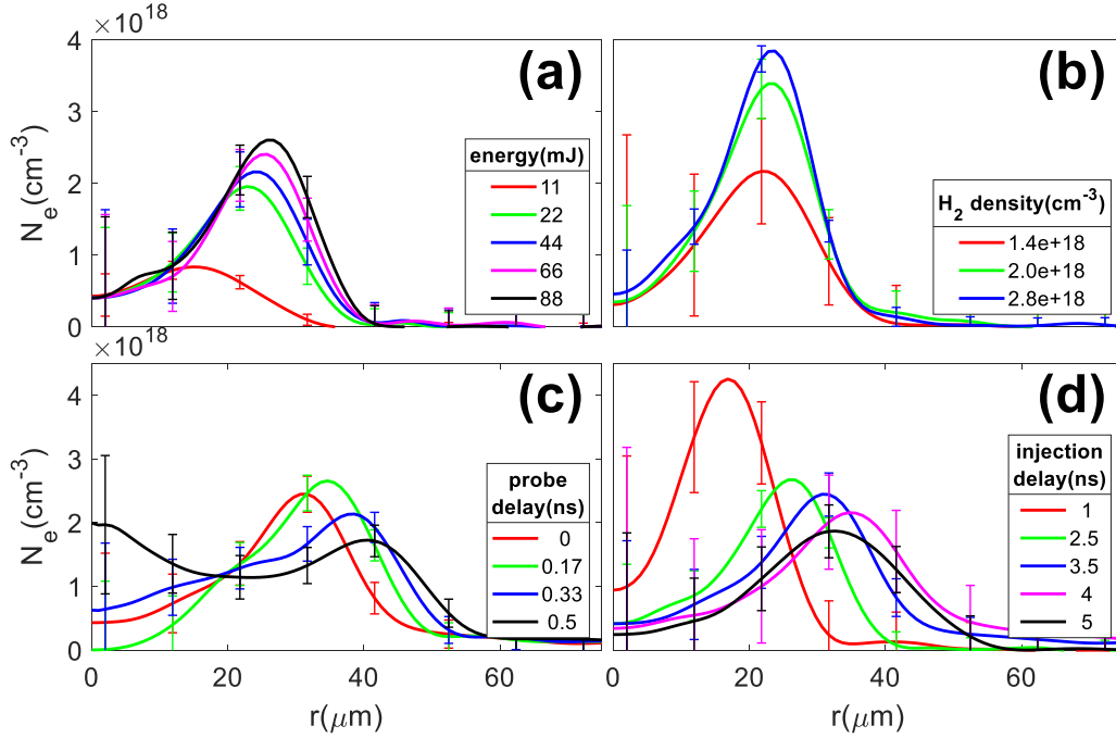
FIG. 3. (a) Electron-density profiles generated at z = 2 cm vs injected pulse energy. \Delta t_{\text{inj}} = 2.5 ns, N_{H_2} = 1.6 \times 10^{18} \text{ cm}^{-3} . (b) \Delta t_{\text{inj}} = 2.5 ns, injection beam energy = 88 mJ. (c) \Delta t_{\text{inj}} = 3.5 ns, N_{H_2} = 1.6 \times 10^{18} \text{ cm}^{-3} , injection beam energy = 88 mJ. (d) N_{H_2} = 1.6 \times 10^{18} \text{ cm}^{-3} , injection beam energy = 88 mJ. All panels: Probe delay (with respect to injection pulse) = 5 ps.
