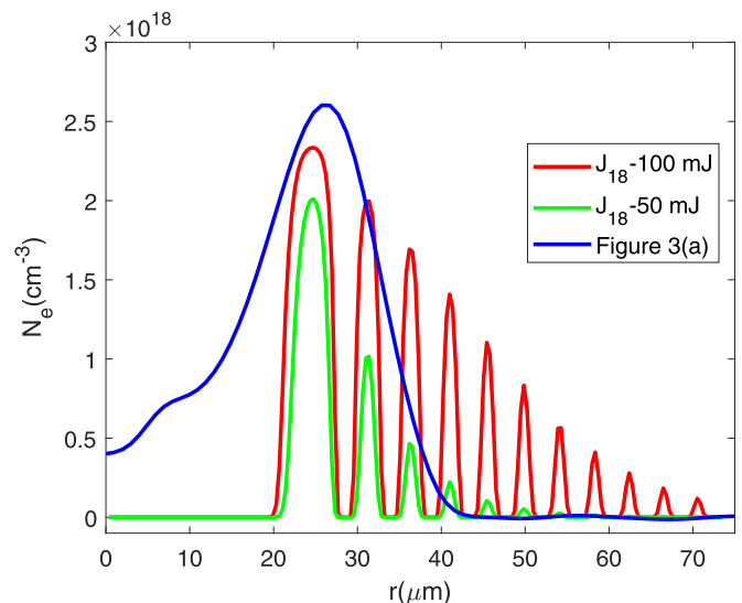
FIG. 10. Energy requirement comparison. Blue curve: Plasma density profile shown in Fig. 3(a) of the main text. Red line: Plasma density profile generated by a J_{18} Bessel beam pulse with 100 mJ energy, assuming a background hydrogen atom density N_H = 2.5 \times 10^{18} \text{ cm}^{-3} . Green line: Plasma density profile generated by a J_{18} Bessel beam with 50 mJ energy with the same background N_H .
