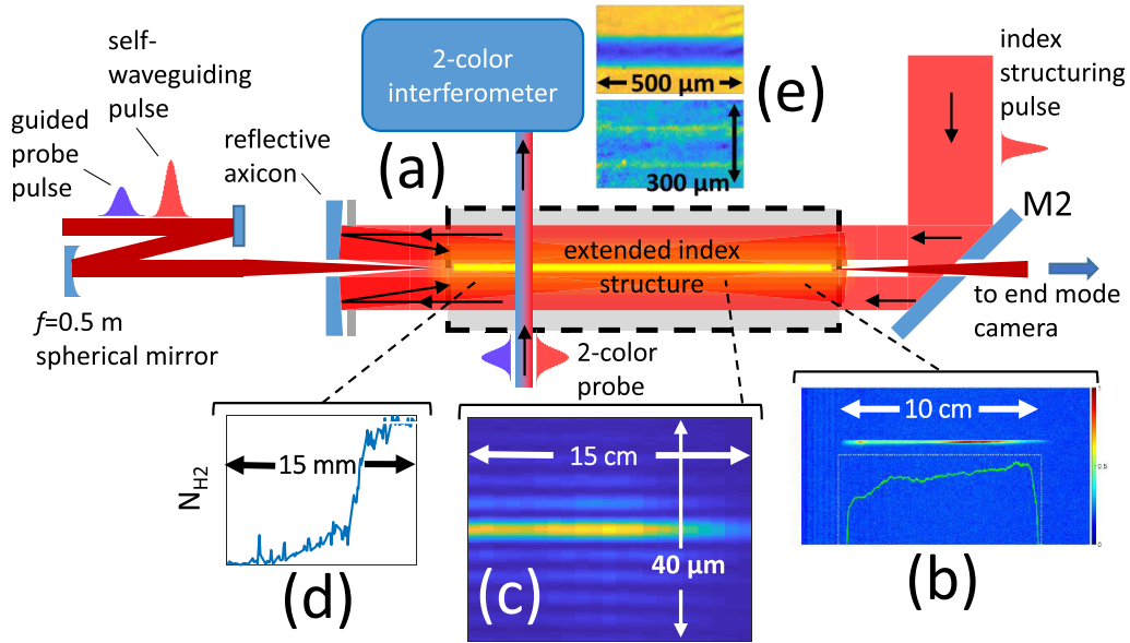
FIG. 1. (a) Experimental setup, showing index structuring Bessel beam pulse ( J_0 pulse) (100 mJ, 75 fs linearly polarized, \lambda = 800 nm) focused by a reflective axicon with base angle \alpha = 3^\circ , over a 10-cm-long supersonic hydrogen gas jet. After a delay \Delta t_{inj} , a 40-fs, 10–90-mJ linearly polarized pulse (self-waveguiding pulse) is focused through a hole in the axicon at f/40 and injected into the entrance of the index structure. The exit of the index structure is imaged by an end-mode CCD camera. A follow-on pulse (guided probe pulse) is guided by the plasma waveguide generated by the self-waveguiding pulse. (b) H_2 gas density profile and fluorescence from plasma recombination after optical-field ionization by the J_0 pulse. (c) Magnified axial scan of the J_0 beam profile. (d) \sim 2 -mm density falloff at the entrance of the jet. (e) Two-color ( \lambda = 400 and 800 nm) interferometric probe pulse is directed transversely through the index structure and into a folded wave-front interferometer, with extracted phase maps from the electron density (top) and neutral (bottom) profiles shown (see Appendix C).
