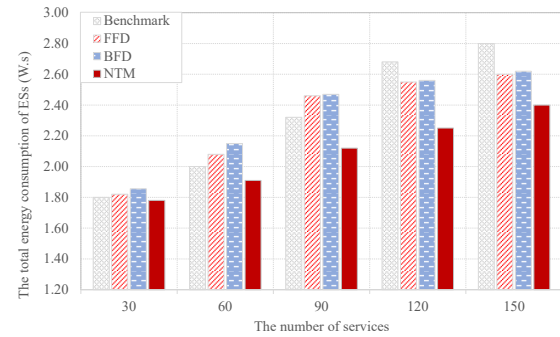
Fig. 6: The total energy consumption of ESs
