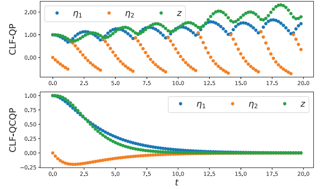
Fig. 1. With inputs applied via a zero-order hold, the (CLF-QP) does not stabilize the system (35) (Top), while the (CLF-QCQP) does (Bottom). Simulation code listed at https://bit.ly/CLF-QCQP .
