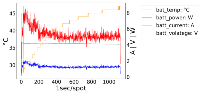
Fig. 9: AR: Battery power consumption and temperature
