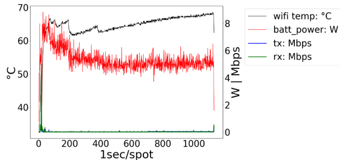
Fig. 13: AR: Power consumption and WiFi chip temperature
