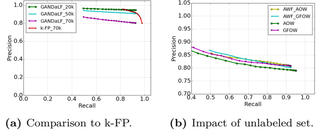
Fig. 5. WF-S, OW: GANDaLF OW experiment by varying the background sizes and unlabeled sets.
