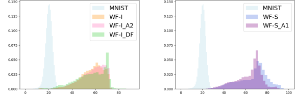
Fig. 3. Distribution of euclidean distances between labeled and unlabeled data (A1: AWF [22] set consisting of 100 websites, A2: AWF set consisting of 100 websites (different from A2), and D: DF set [25]).
