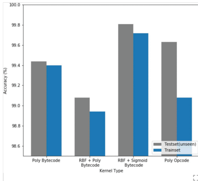
Fig. 4. Detection accuracy of different combinations of SVM kernels on the test and train data set.
