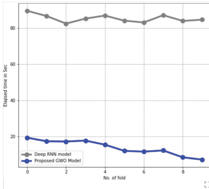
Fig. 8. Comparison of training and testing time between the proposed model and a deep RNN during convergence.
