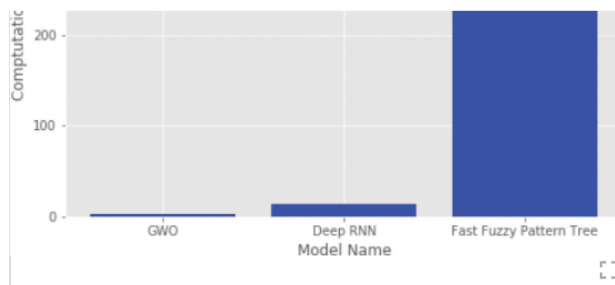
Fig. 9. Comparison of the overall computational time of the proposed model with previous deep RNN and fuzzy pattern tree models.
