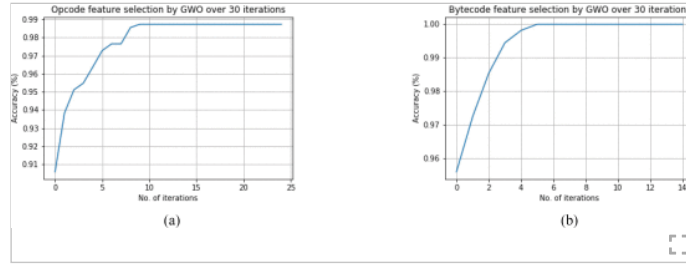
Fig. 2. (a) Detection accuracy in Opcode by GWO over 30 iterations. (b) Detection accuracy of the selected features in Bytecode by GWO over 30 iterations.
