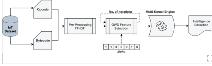
Fig. 1. Proposed model based on an SVM multikernel engine
