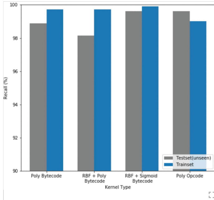
Fig. 6. Recall rates of different combinations of kernels on test and train data set.
