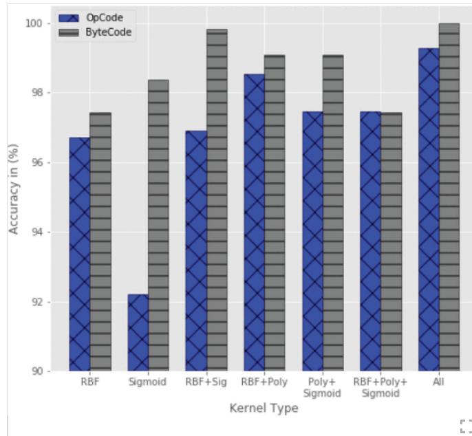
Fig. 7. Overall detection accuracy of the combination of kernels on the unseen malware data set.
