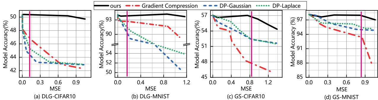
Figure 5. Compared defenses on model accuracy and MSE between reconstructed image and raw image for different attack baselines and datasets. The pink vertical line is the boundary that the reconstructed image is unrecognizable by human eyes if MSE is higher.
