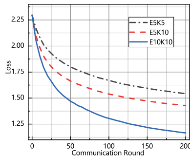
Figure 7. Convergence of LR+FedAvg with our defense.
