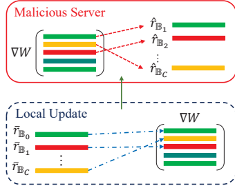
Figure 2. Illustration of our representation inference algorithm.
