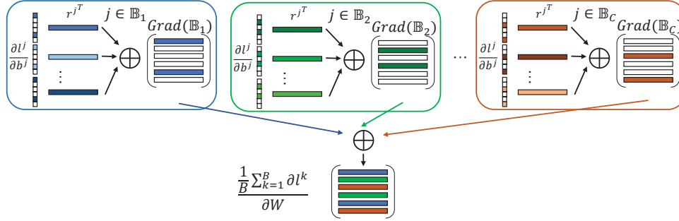
Figure 1. Illustration of the gradient updates of class-wise data in a batch.
