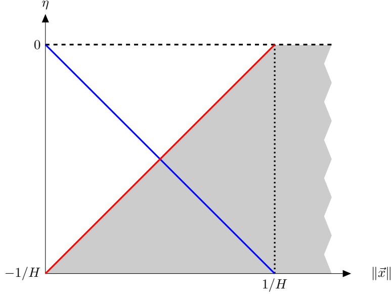
Figure 2: Conformal diagram of the cosmological patch of de Sitter space. The system is released at time \eta_0 = -1/H , with a scalar point source at the origin \vec{x} = 0 . The asymptotic future corresponds to the \eta = 0 slice. The red line denotes the light cone of the point source given by (\eta - \eta_0) - \|\vec{x}\| = 0 , while the blue line denotes the Hubble distance from the source given by aH\|\vec{x}\| = 1 , which coincides with the past particle horizon of a distant future observer at the origin. We are interested in the effects within the light cone (nonshaded region) which capture the dynamical effects of graviton loops.
