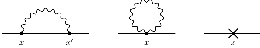
Figure 1: One-particle-irreducible diagrams contributing to the scalar self-mass-squared at the one-loop order. The solid lines stand for the scalar and wavy ones for the graviton. The rightmost diagram stands for the counter-terms.
