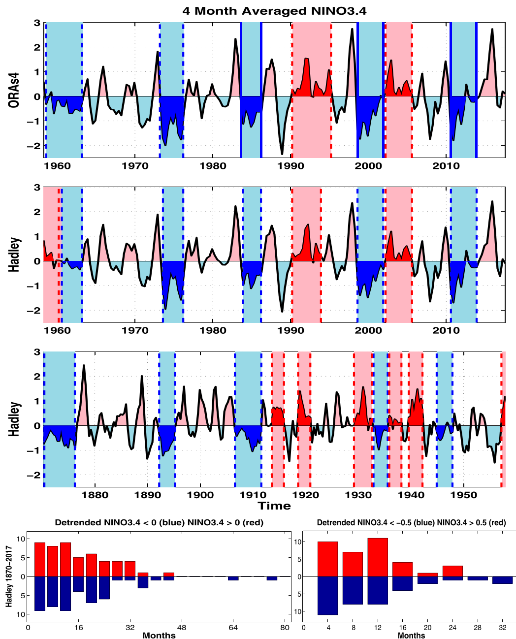
FIG. 1. The Niño-3.4 SST index in non-overlapping 4-month averages (top) from June 1958 to September 2017 from ECMWF and (top middle), (bottom middle) from June 1870 to September 2017 from Hadley Centre data. The persistent cold states, defined as periods of more than 30 months with no more than one 4-month period within that has an above-zero Niño-3.4 value, are marked between dashed and solid vertical lines with blue shading in between. Similarly identified warm states are marked by vertical lines and red shading. The solid lines denote the three cold states in the post-1979 period studied using the ECMWF data. (bottom) Counts with the detrended longer Hadley data of cold (below the zero x axis and blue) and warm (above the zero x axis and red) states of the length in months indicated using the deviation from (left) a 0^{\circ}\text{C} criterion and (right) below -0.5^{\circ} and above 0.5^{\circ}\text{C} criteria.
