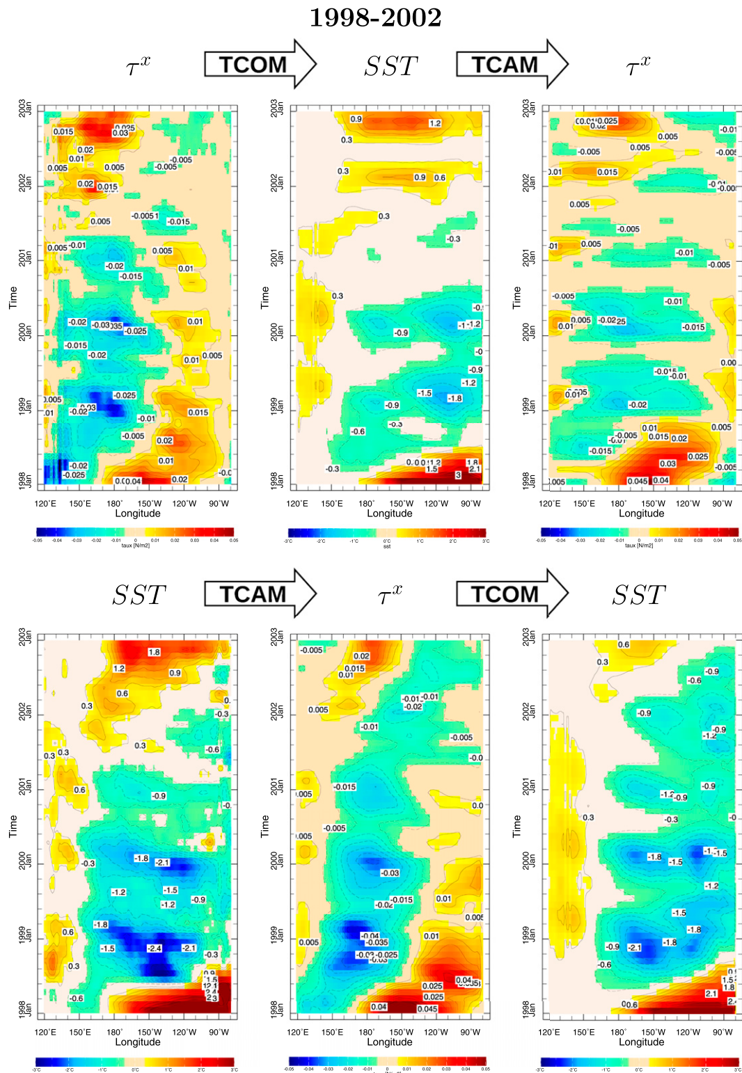
FIG. 11. As in Fig. 10, but for the 1998–2002 cold state.
