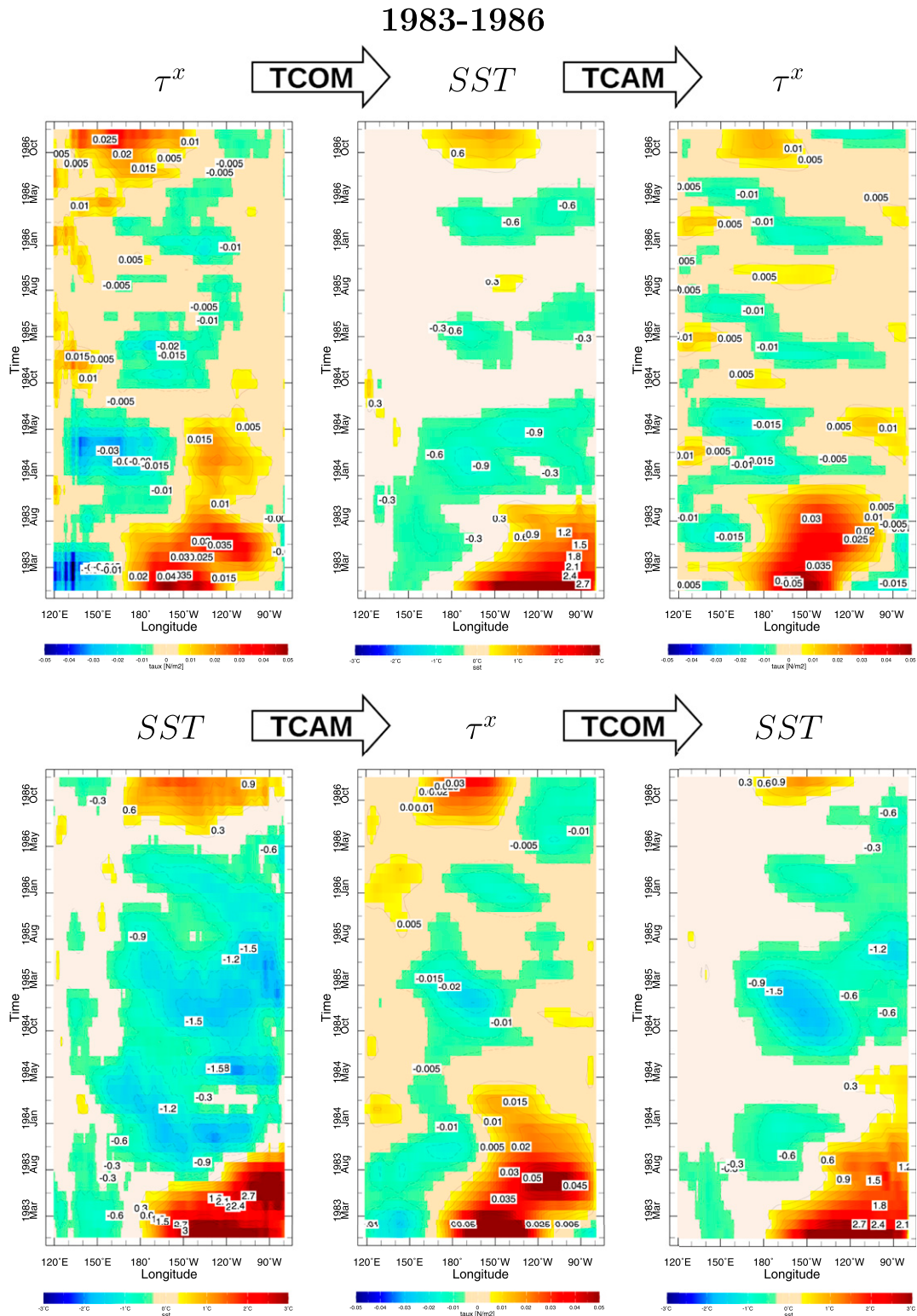
FIG. 10. Ocean and atmosphere modeling results for the 1983–86 cold state. (top, from left to right) The ECMWF zonal wind stress, the SST produced by the ocean model with simplified SST equation forced by this wind stress, and the zonal wind stress computed by the atmosphere model forced by the ocean model SST. (bottom, from left to right) The ECMWF SST, the zonal wind stress simulated by the atmosphere model forced by this SST, and the SST simulated by the ocean model and simplified SST equation when forced by the atmosphere model zonal wind stress.
