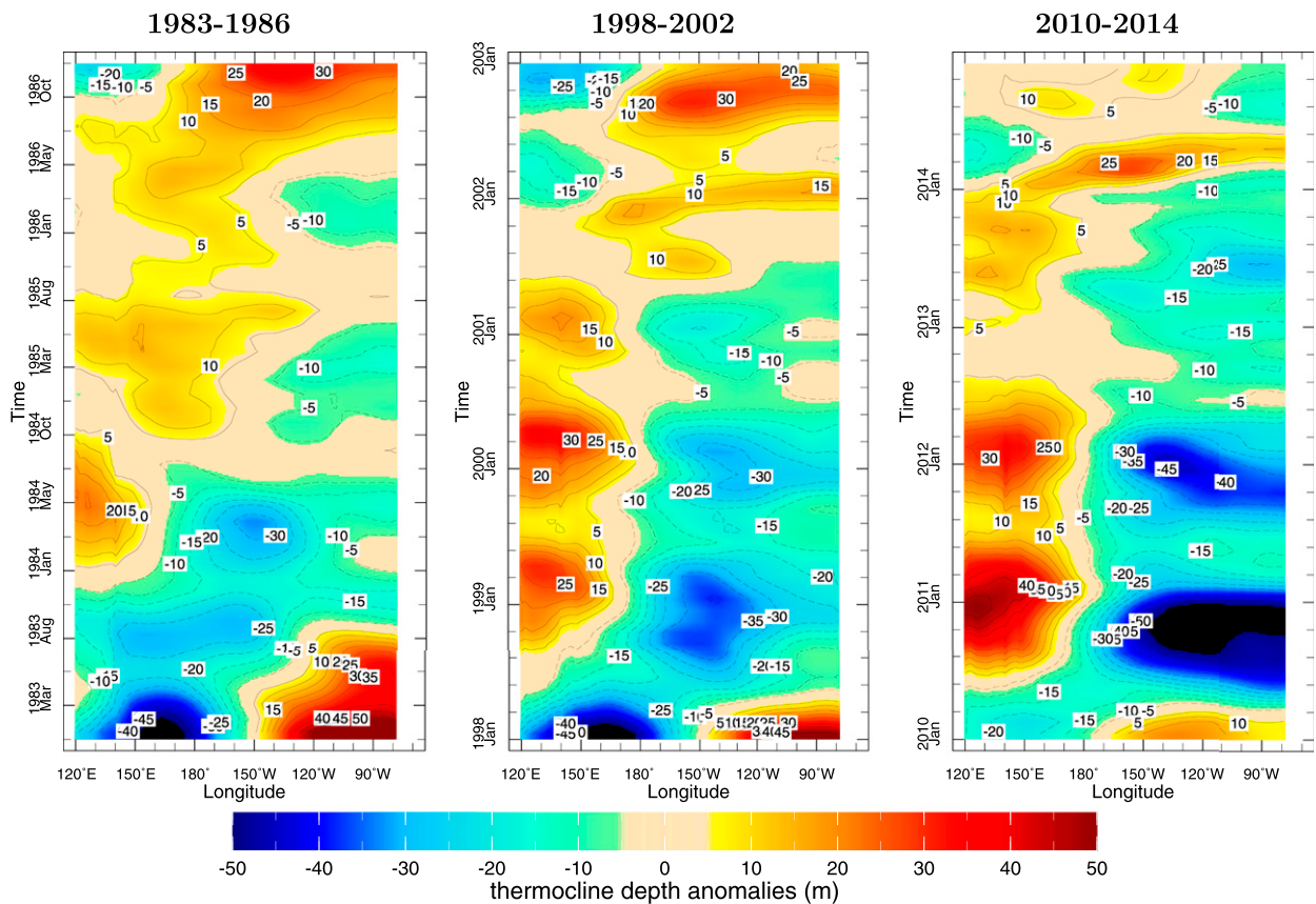
FIG. 7. The thermocline depth anomalies (m) simulated by the ocean model with global wind stress forcing (contours) and equatorial zonal wind stress anomalies only (colors).
