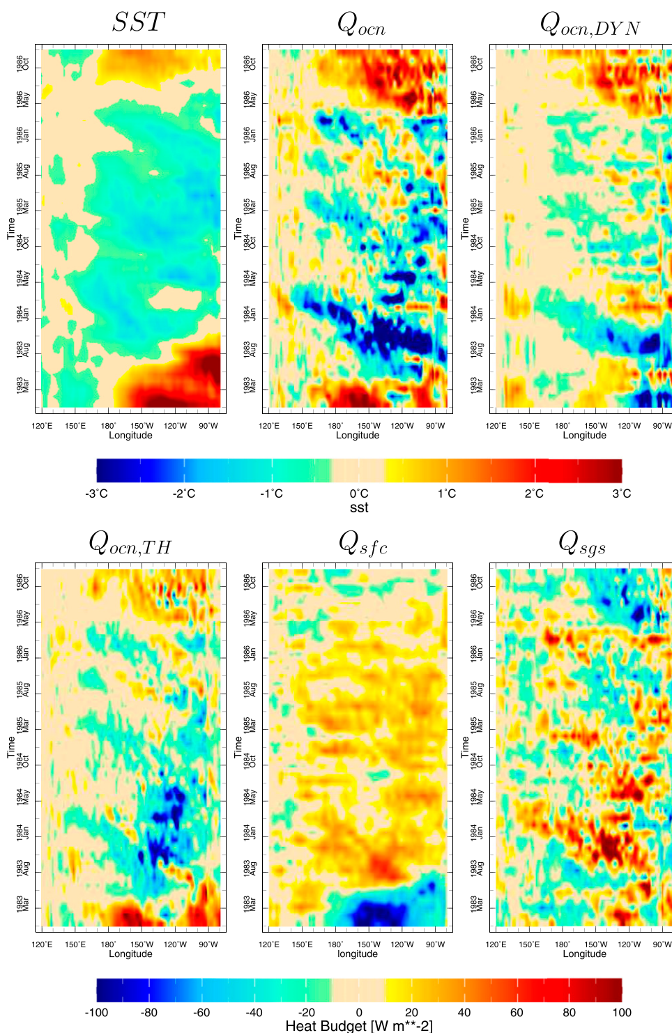
FIG. 4. Hovmöller plots of ECMWF SST and components of the upper-50-m ocean heat budget during the 1983–86 cold state. Shown are (top left) SST (K) and (top center) heat content tendency ( W m^{-2} ) due to ocean heat transport convergence, and their decomposition into components due to (top right) circulation change and (bottom left) ocean temperature change, (bottom middle) net surface heat flux, and (bottom right) subgrid-scale processes.
