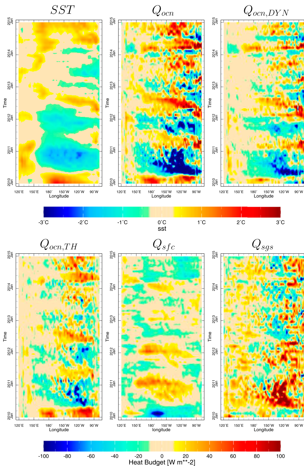
FIG. 6. As in Fig. 4, but for the 2010–14 cold state.
