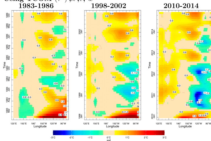
FIG. 8. Simplified models of the cold states. (top) Using currents and T_{50} from ECMWF in the simplified SST equation, which is integrated forward from ECMWF initial conditions on 1 Jan of the first year of the cold state. (middle) Replacing ECMWF currents and T_{50} with those from the ocean model driven only by equatorial zonal wind stress anomalies. (bottom) Replacing the zonal current anomaly with that calculated from a balance of Rayleigh friction and zonal wind stress.
