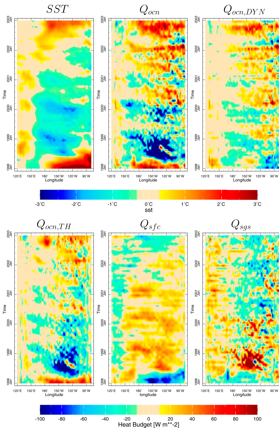
FIG. 5. As in Fig. 4, but for the 1998–2002 cold state.
