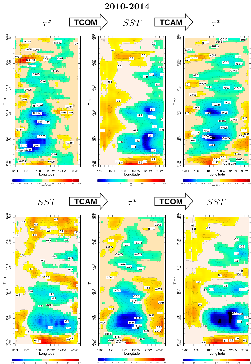
FIG. 12. As in Fig. 10, but for the 2010–14 cold state.
