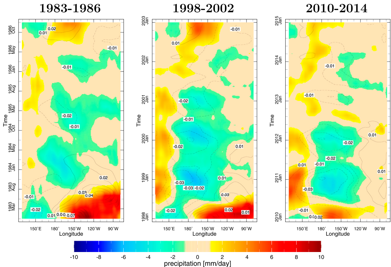
FIG. 9. The precipitation (color) and zonal wind stress (contours) anomalies computed by the atmosphere model forced by ECMWF SSTs for the three cold states.
