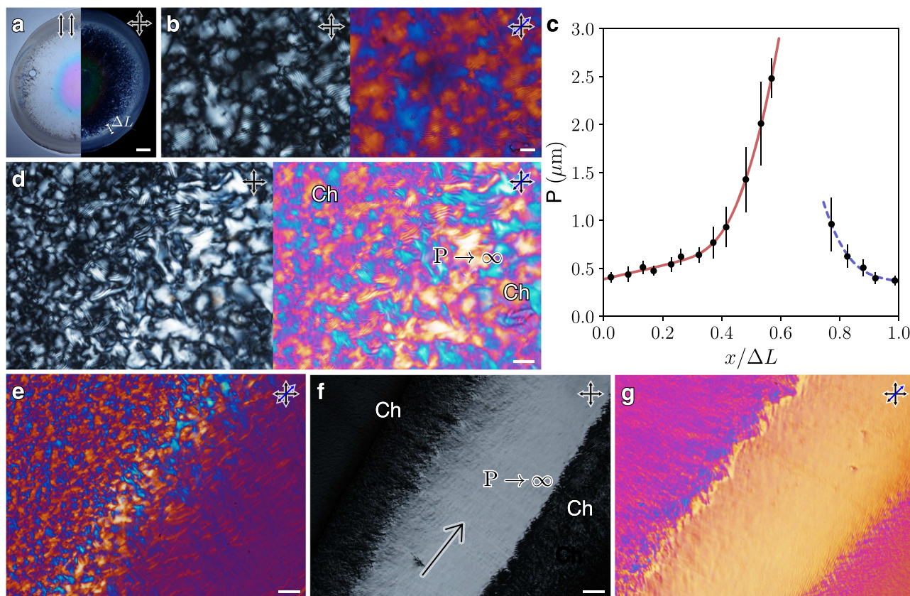
Fig. 2 Evidence of the nematic phase between left (L) and right (R) helicoidal structures. a Photo of a quasi-2D sample illuminated under white light between parallel (on the left) and cross polarisers (on the right). b POM pictures taken in transmission, between cross polarisers (on the left) and between crossed polarisers with a lambda plate (on the right), showing cholesteric domains with fingerprint textures, taken in region \Delta L (shown in a ). c Dependence of the pitch with distance ( x ) along \Delta L (shown in a ). POM pictures taken in transmission, between cross polarisers ( d (left), f ) and between crossed polarisers with a lambda plate ( d (right), e , g ), at values of x/\Delta L \approx 0.6 . The sample was sheared (shear direction arrow in f ) evidencing different optical axis alignment of the liquid crystalline phases, parallel and perpendicular, to the "slow axis" of the red plate (in g ), for the cholesteric (Ch) and the nematic (N) phases, respectively. Scale bars in a 2 mm, in b 10 \mu\text{m} , in d 20 \mu\text{m} and in e 50 \mu\text{m} and f , g 100 \mu\text{m} .
