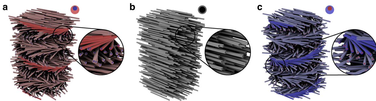
Fig. 6 Idealised structures of the left, nematic and right structures formed by self-assembled cellulosic chains (rods). a Left-handed helicoidal structures formed by rods (cross-section shown in the upper right corner) that expose hydrophobic groups of cellulose (red colour) and hide the hydrophilic groups (blue colour) asymmetrically from the interface, along the rods, due to the chirality of the cellulose main chain. b Nematic structure formed by symmetric rods (cross-section in the upper right corner). c Right-handed helicoidal structures formed by rods (cross-section shown in the upper right corner) that expose cellulose hydrophilic groups (blue colour) and hide the hydrophobic groups (red colour) asymmetrically along the rods.
