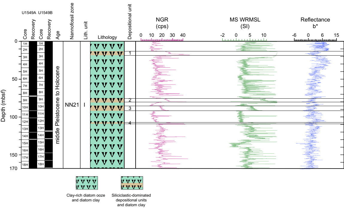
Figure F12. Lithostratigraphic column, Site U1549. NGR = natural gamma radiation, cps = counts per second, MS = magnetic susceptibility, WRMSL = Whole-Round Multisensor Logger.
