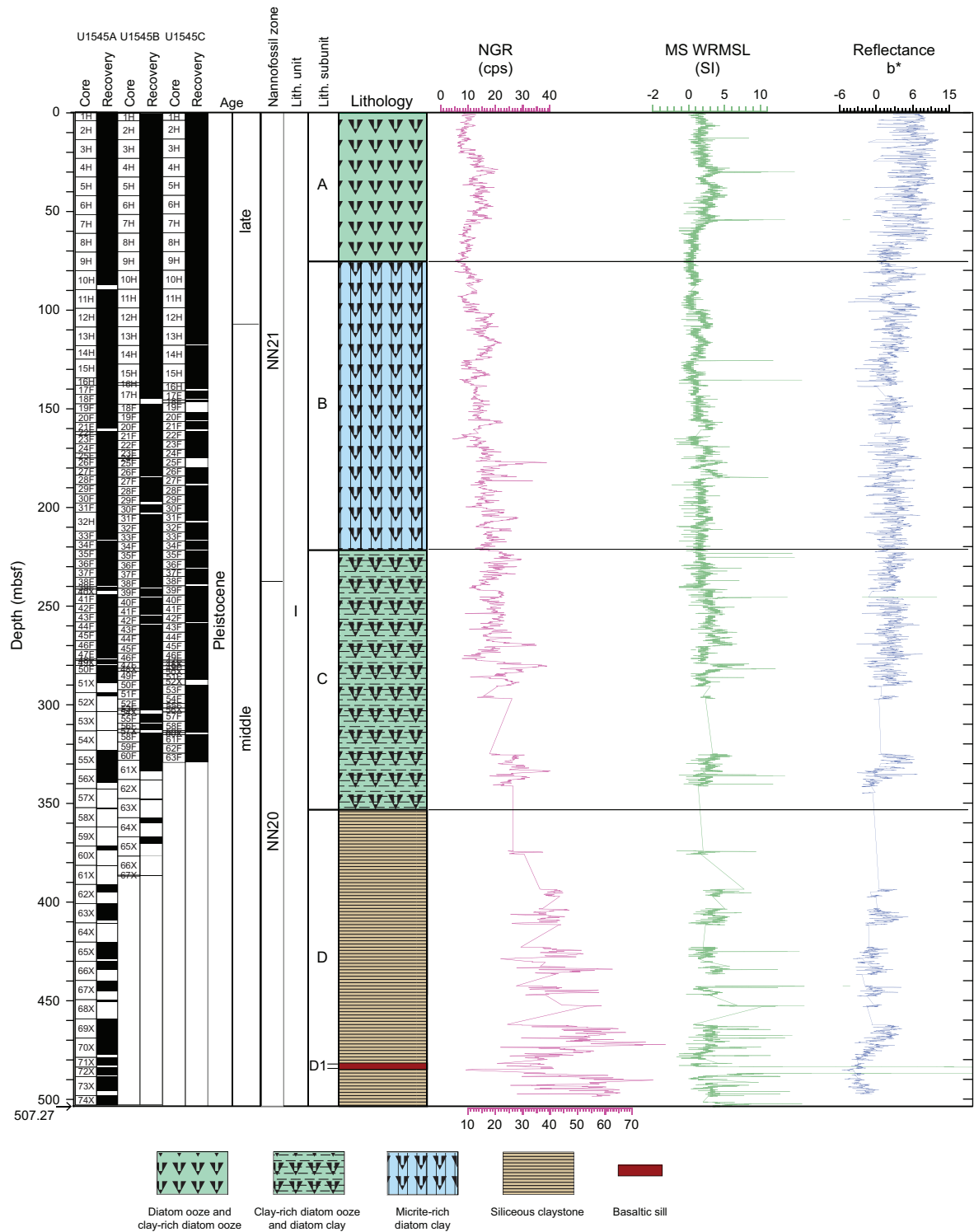
Figure F5. Lithostratigraphic column, Site U1545. NGR = natural gamma radiation, cps = counts per second, MS = magnetic susceptibility, WRMSL = Whole-Round Multisensor Logger. Reflectance b*
