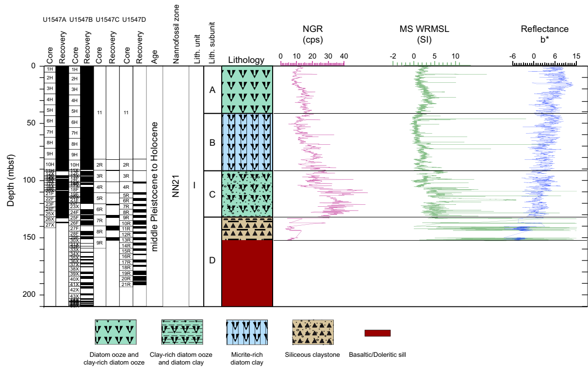
Figure F8. Lithostratigraphic column, Site U1547. NGR = natural gamma radiation, cps = counts per second, MS = magnetic susceptibility, WRMSL = Whole-Round Multisensor Logger.
