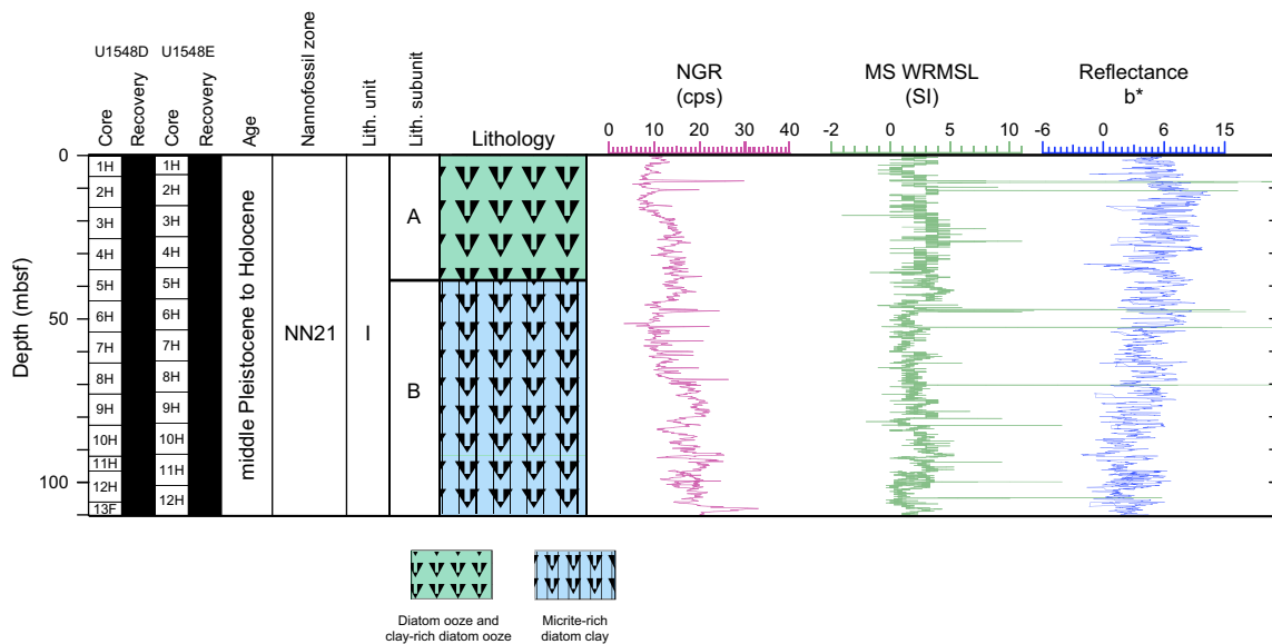
Figure F10. Lithostratigraphic column, Holes U1548D and U1548E. NGR = natural gamma radiation, cps = counts per second, MS = magnetic susceptibility, WRMSL = Whole-Round Multisensor Logger.
