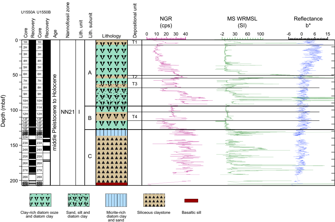
Figure F14. Lithostratigraphic column, Site U1550. NGR = natural gamma radiation, cps = counts per second, MS = magnetic susceptibility, WRMSL = Whole-Round Multisensor Logger.
