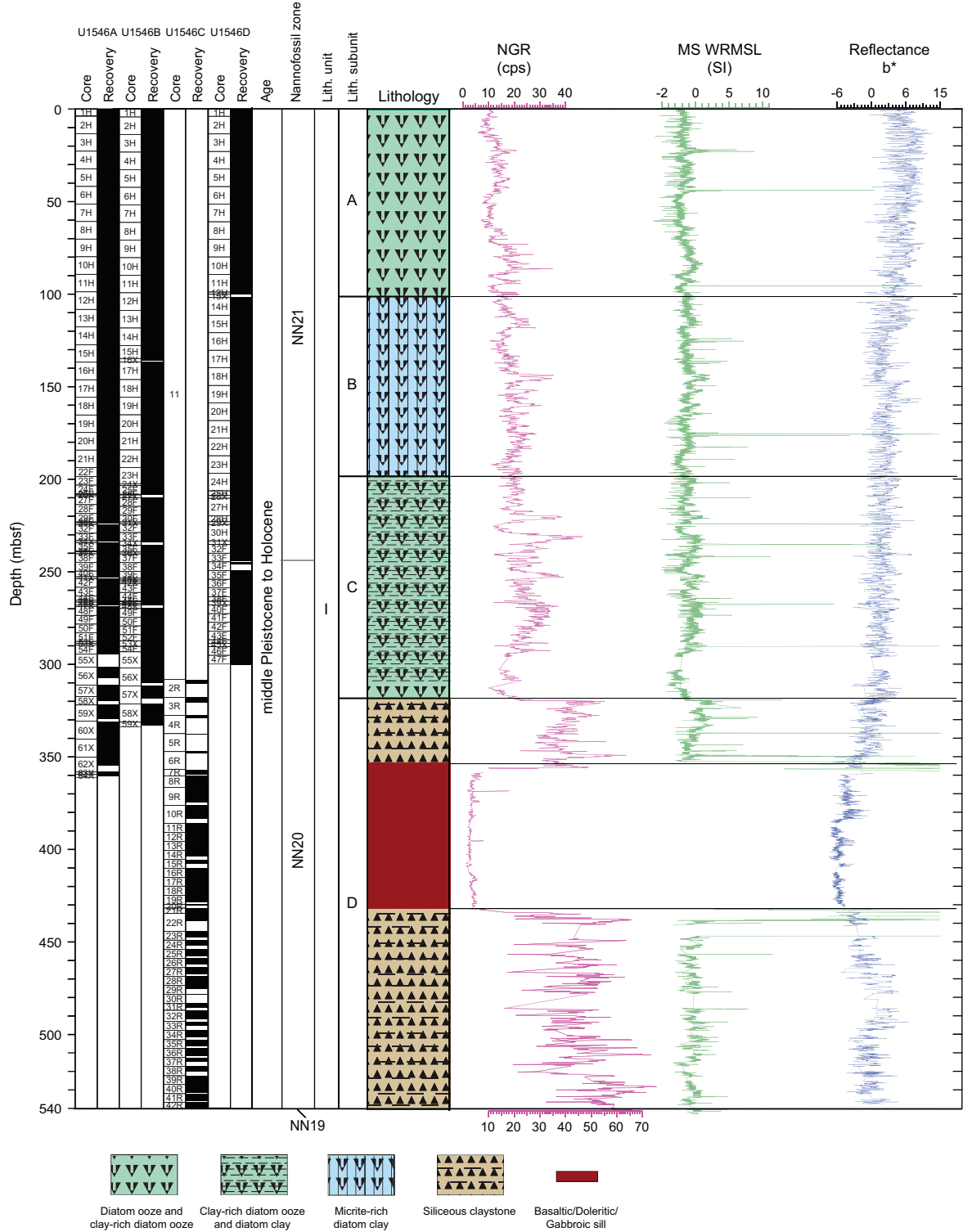
Figure F6. Lithostratigraphic column, Site U1546. NGR = natural gamma radiation, cps = counts per second, MS = magnetic susceptibility, WRMSL = Whole-Round Multisensor Logger.
