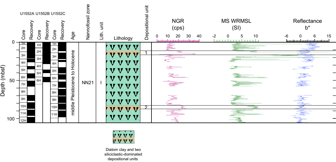
Figure F18. Lithostratigraphic column, Site U1552. NGR = natural gamma radiation, cps = counts per second, MS = magnetic susceptibility, WRMSL = Whole-Round Multisensor Logger.
