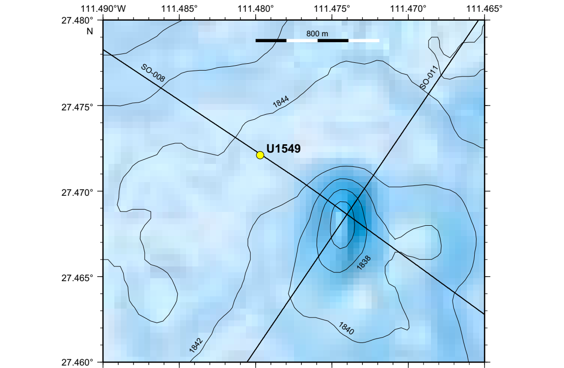
Figure F11. Bathymetric map showing Site U1549, which is situated along Seismic Line SO-008 approximately 700 m northwest of a seafloor mound where cold-seep fauna exists. The locations of drilled holes are not distinguishable at the given scale. Contour lines = 2 m.
