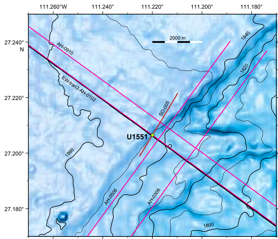
Figure F15. Bathymetric map of Site U1551 and its surrounding area. Multiple pre-cruise seismic lines, including EW-tran3, are also shown. The seafloor bathymetry reflects the mode of predominant mass-gravity sediment deposition. Site U1551 is sited at the edge of a large slide deposit that is imaged in the seismic data. The locations of drilled holes are not distinguishable at the given scale. Contour lines = 10 m.
