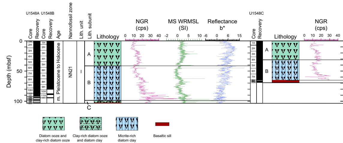
Figure F9. Lithostratigraphic column, Holes U1548A–U1548C. NGR = natural gamma radiation, cps = counts per second, MS = magnetic susceptibility, WRMSL = Whole-Round Multisensor Logger.
