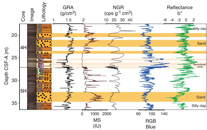
Figure F55. Characteristic variations in major lithology and physical properties, Hole U1544A. Orange bars = sand (Lithofacies 11), pale orange bars = nanno-fossil ooze (Lithofacies 4 and 10), white bars = diatom ooze (Lithofacies 6) and siliciclastic sediments (Lithofacies 7 and 8).
