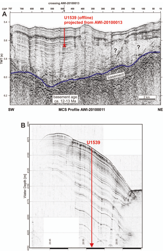
Figure F13. (A) Multichannel seismic and (B) Parasound profiles, Site U1539.
