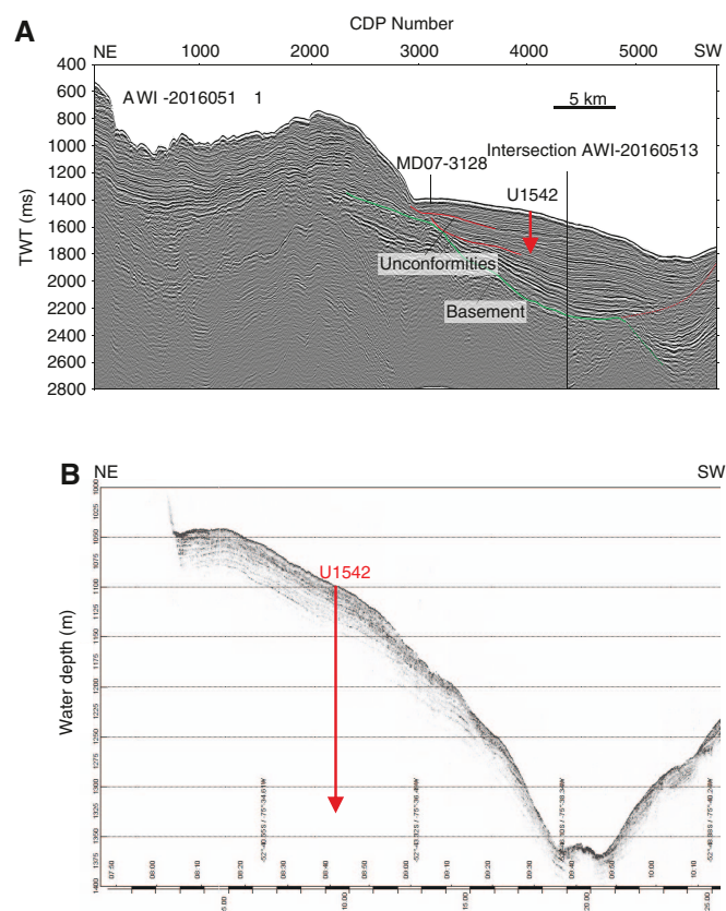
Figure F36. (A) Multichannel seismic and (B) Parasound profiles, Site U1542. TWT = two-way traveltime, CDP = common depth point.
