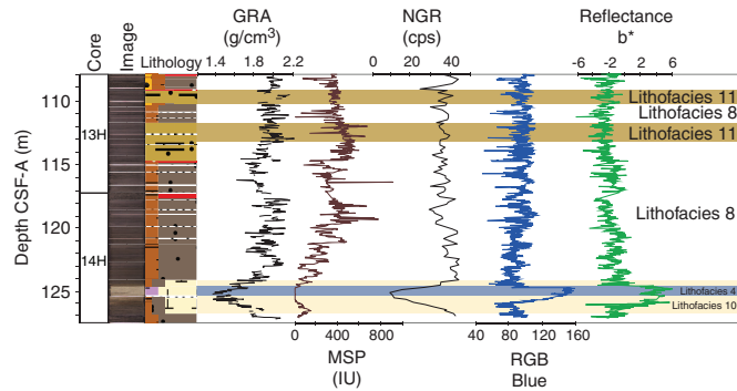
Figure F41. Characteristic variations in major lithology and physical properties, Hole U1542C. GRA = gamma ray attenuation bulk density, MSP = point magnetic susceptibility, NGR = natural gamma radiation, RGB = red green blue.
