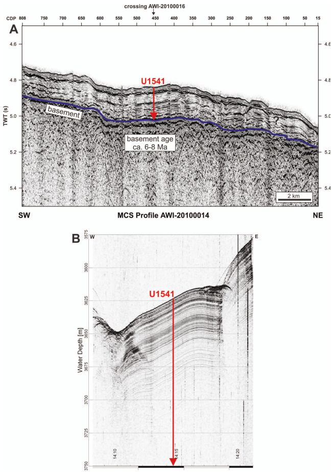
Figure F28. (A) Multichannel seismic and (B) Parasound profiles, Site U1541. TWT = two-way traveltime, CDP = common depth point.
