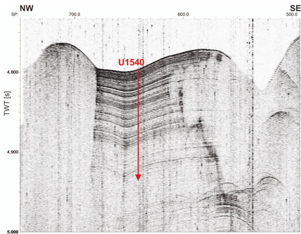
Figure F21. Parasound profile, Site U1540. TWT = two-way traveltimes, SP = shot point.
