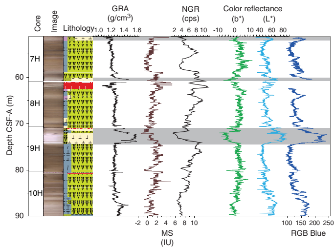
Figure F18. Characteristic variations in major lithology with changes in natural gamma ray (NGR), gamma ray attenuation (GRA) bulk density, magnetic susceptibility (MS), sediment color reflectance (b* and L*), and the RGB blue value, Hole U1539A. Lithologies are determined by visual core description, smear slide analyses, and X-ray imaging. Gray bars show intervals of light-colored nannofossil ooze.
