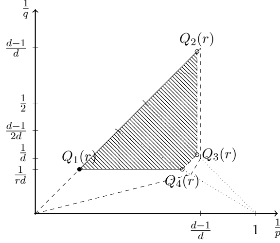
FIGURE 3. The quadrangle \mathfrak{Q}_d(r) for 1 \leq r \leq \frac{d}{d-1} and d \geq 4 (Theorem 1.5). The outer (dashed) quadrangle is the bound- edness region for the maximal function. Shown with d = 4 and r = \frac{5}{4} .
