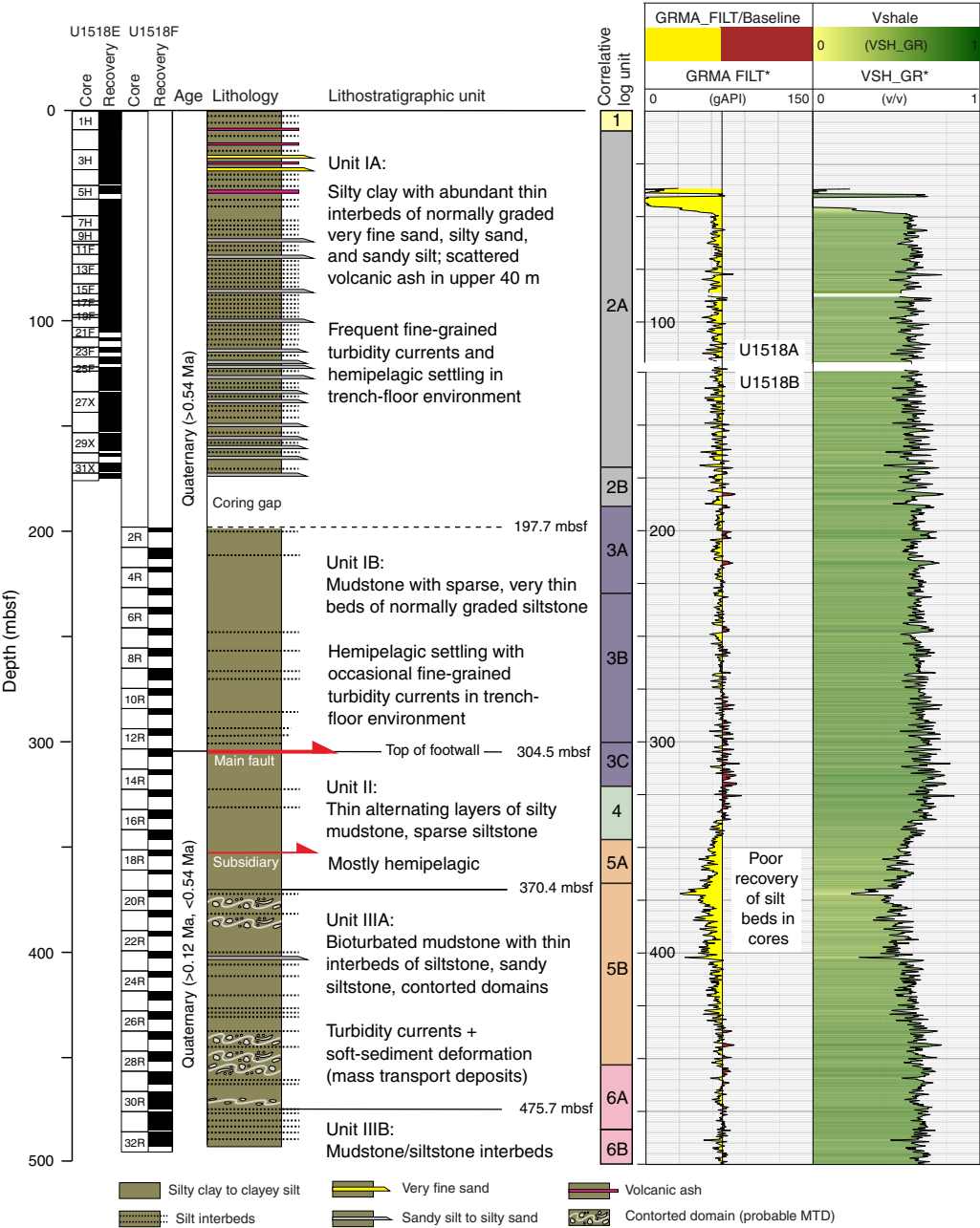
Figure F6. Stratigraphic column, Site U1518. Filtered gamma ray data are from LWD acquired during Expedition 372. Vshale = shale content estimates.
