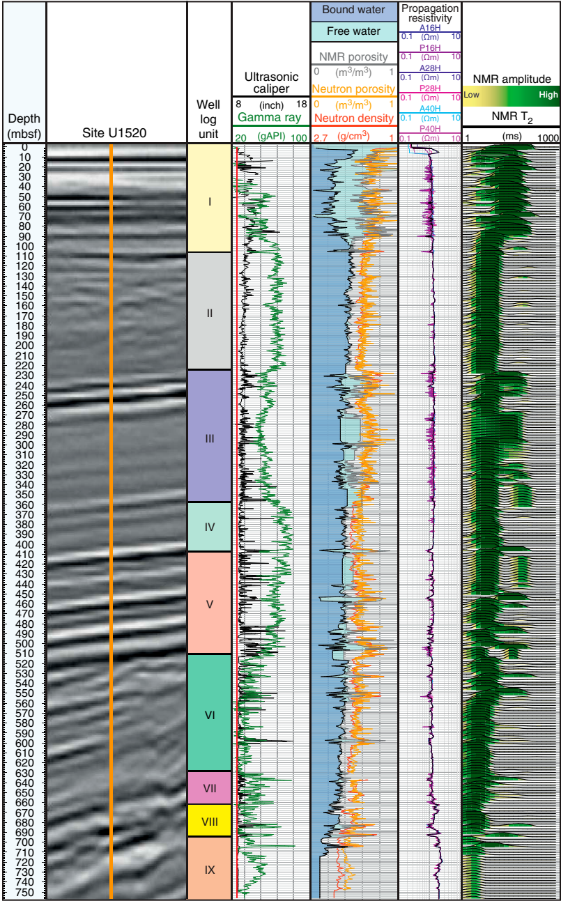
Figure F14. Composite plot of seismic image (05CM-04) and selected measurements from LWD, Site U1520. PSDM seismic section was provided by GNS Science, New Zealand.
