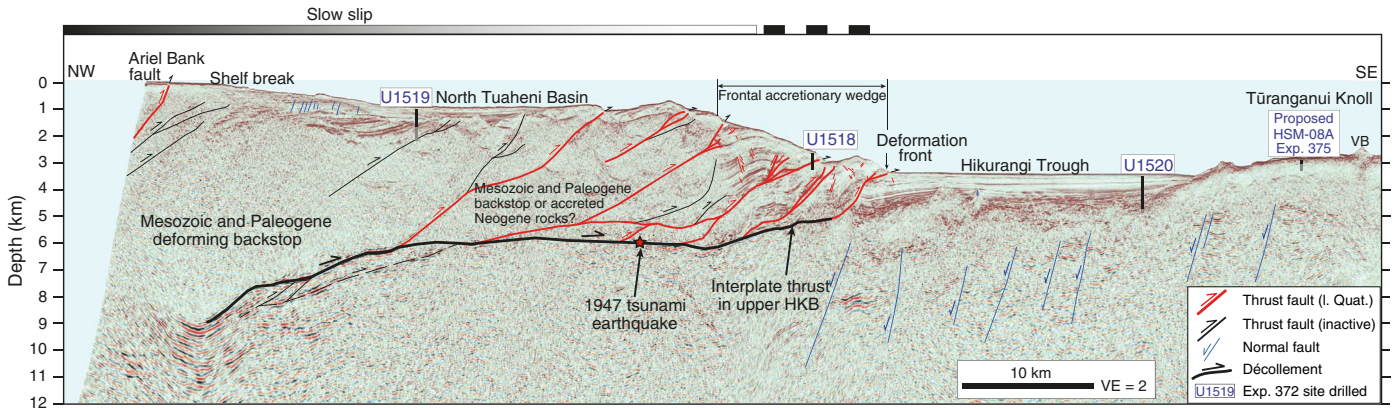
Figure F3. Interpretation of regional depth-converted seismic Profile 05CM-04 showing major faults and HSM site locations. HKB = Hikurangi Basement Sequence. Seismic depth section was provided by GNS Science, New Zealand. VE = vertical exaggeration.
