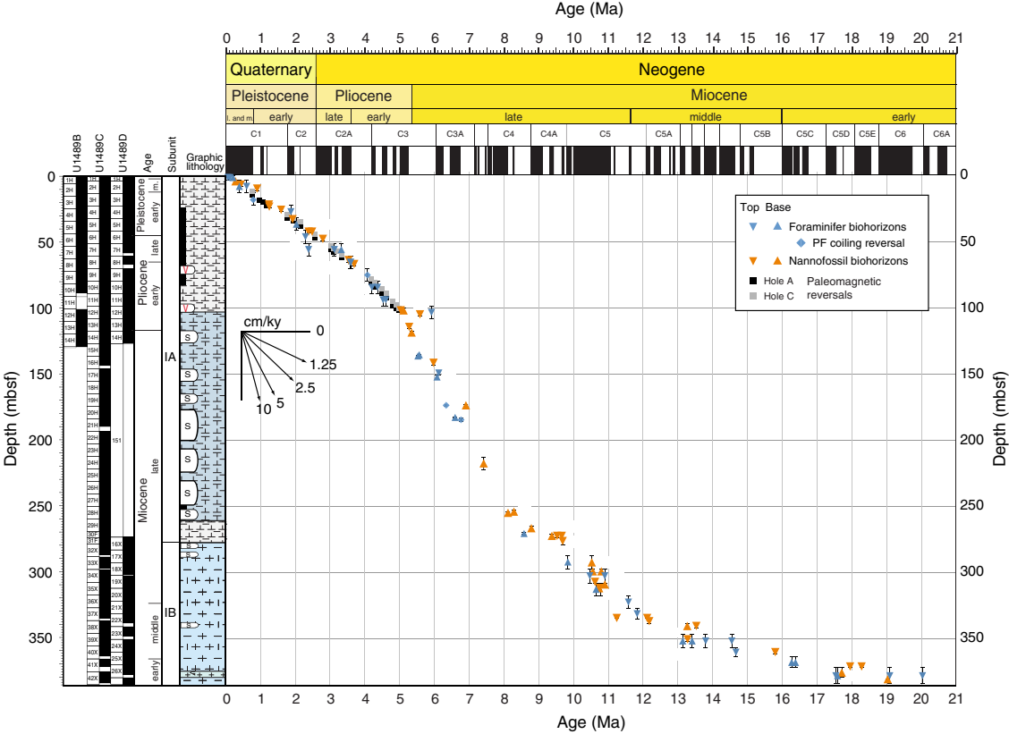
Figure F25. Age-depth plot for Site U1489 showing integrated biomagnetochronology in Hole U1489C. The stratigraphy of the base of Hole U1489C is constrained by biohorizon base Sphenolithus belemnus (19.03 Ma) and by the presence of Dentoglobigerina binaiensis (>19.30 Ma) and absence of Globigerinoides altiaperturus (>20.03 Ma) and Tenuitella munda (<20.78 Ma) at ~380 mbsf. Average sedimentation rates vary from ~0.3 to 5 cm/ky. PF = planktonic foraminifer.
