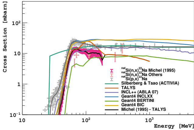
FIG. 3. Experimental measurements (magenta and pink error bars) [45, 58–61] and model estimates (continuous curves) of the neutron-induced ^{22}\text{Na} production cross section in silicon. Measurements of the proton-induced cross section [46, 47] are also shown for reference (gray error bars).
