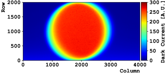
FIG. 10. Post-irradiation dark-current profile for CCD3, obtained from the median pixel values across multiple images. The elevated number of dark counts in the center of the CCD shows the effect of the neutron damage on the CCD.
