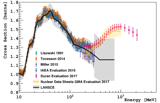
FIG. 8. Experimental measurements (circles) [67, 69, 71] and evaluations (squares) [68, 70, 72, 73] of the ^{238}\text{U}(n, f) cross section. The cross section assumed by the LANSCE facility to convert the fission chamber counts to a total neutron fluence is shown by the black line, with the shaded grey band indicating the assumed uncertainty.
