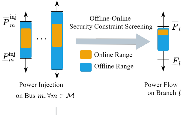
Fig. 1: From Net Power Injection Interval to Power Flow Interval in Offline-online Security Constraint Screening.
