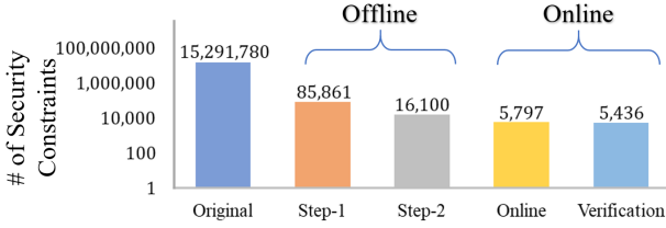
Fig. 6: Screening Performance on MISO Case 11
