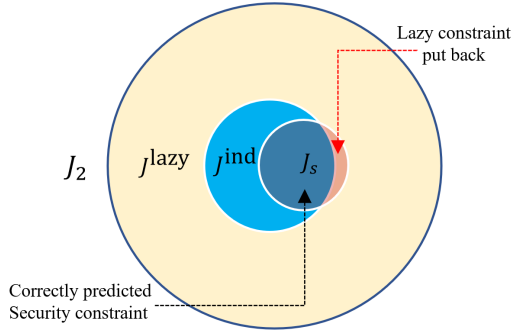
Fig. 4: Relationship between Industrious Constraints J^{\text{ind}} , Lazy Constraints J^{\text{lazy}} and Supporting Constraints J_s
