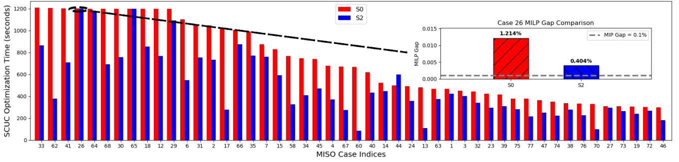
Fig. 9: Comparison of Solution Time with and without Proposed screening. MILP Gaps for Case 26 Are Compared.
