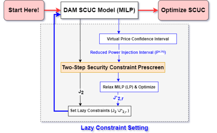
Fig. 5: Incorporating Virtual Price Confidence Interval and Lazy Constraint Setting in DAM SCUC
