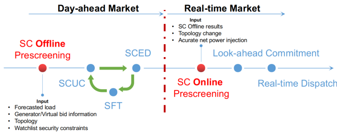
Fig. 2: Offline-online Approach Timeline. SCED: Security Constraint Economic Dispatch, SFT: Simultaneous Feasibility Test.
