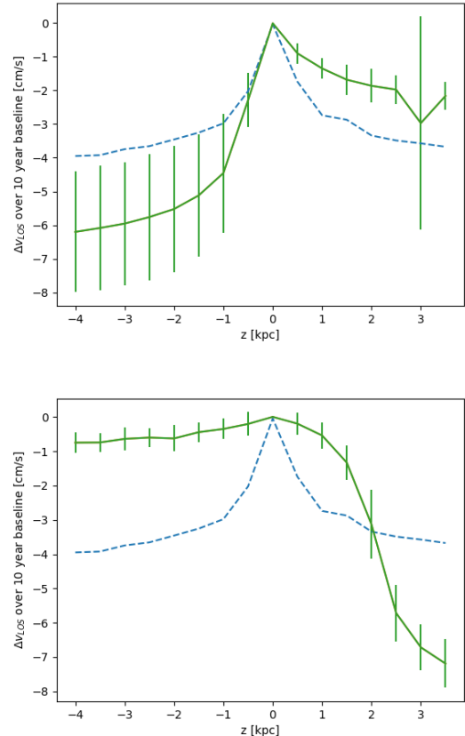
FIG. 2.— (a) Change in the line-of-sight velocity for a simulation of Milky Way interacting with the Antlia 2 dwarf galaxy at present day (solid line) and at early times prior to the interaction with Antlia 2 (dashed line) (Chakrabarti et al. 2019); solid line shows the average over a ring of radius r = 8 kpc, and the error bars show the standard deviation along the azimuth (b) \Delta v_{LOS,z} for the interaction of the Sagittarius dwarf galaxy with the Milky Way (Chakrabarti et al. 2019), with the dashed line displaying the acceleration profile at early times, and the solid line corresponding to the present day.
