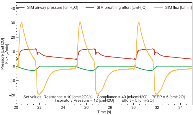
FIG. 9. Example waveforms from the breathing simulator with the MVM in PSV mode.
