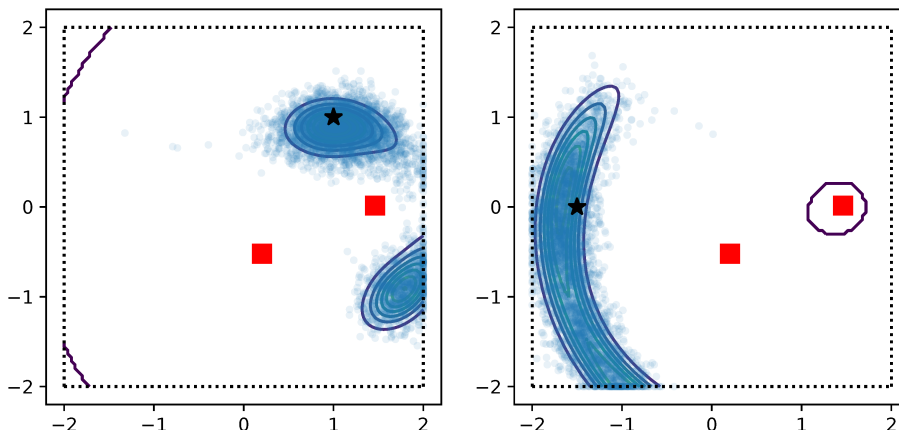
Figure 1: The figures depict two runs of the projected Langevin method for measurements taken from different locations. The black star depicts the sensor location, the red squares are the beacon locations. The dots represent the positions traversed by the algorithm and the contours lines represent the numerically computed posterior density. As can be seen, the method accurately samples from the posterior while satisfying the constraints.
