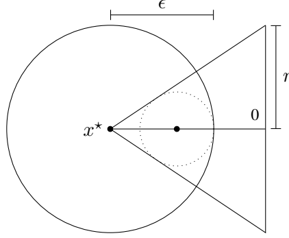
Figure 2: Case of 0 \notin \mathcal{B}_{x^*}(\epsilon) . Using elementary trigonometry the largest inscribed circle can be calculated.
