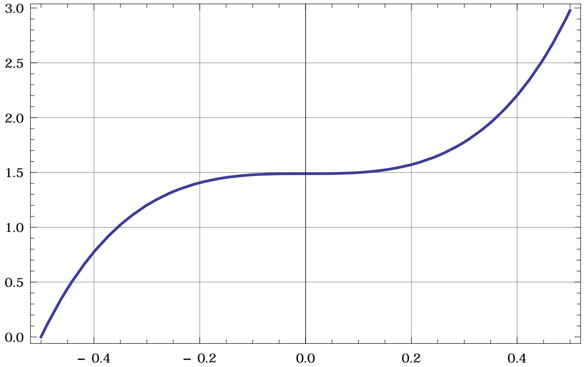
Figure 6: A plot of the function \alpha(t) - ct , where \alpha is nonoscillatory phase function associated with equation (260), c = 10^5 , n = 63769 , and \chi_{n,c} = 1.00060408908491 \times 10^{10} .
