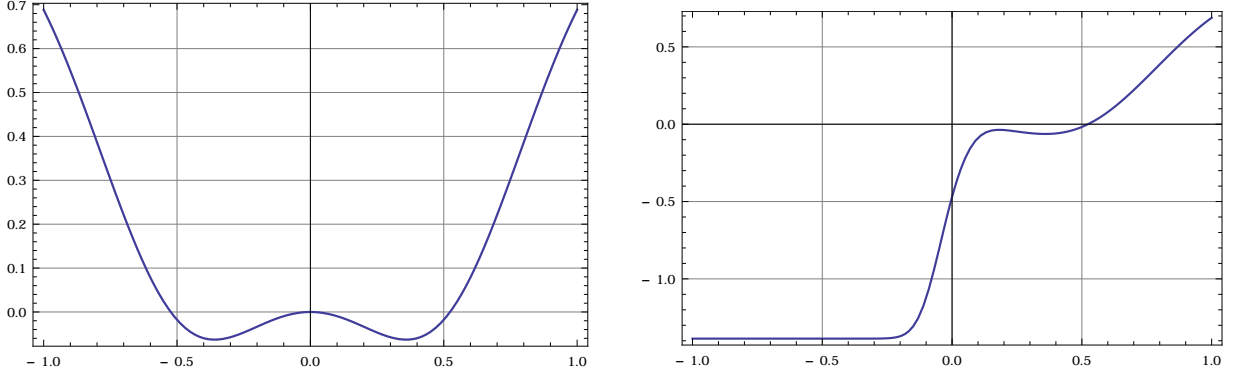
Figure 2: Plots of the solution r of the logarithm form of Kummer's equation associated with the ordinary differential equation (237) in Section 5.1 when \lambda = 10^7 (left) and the function r_1 constructed as an intermediate step by the algorithm of Section 4 (right).
