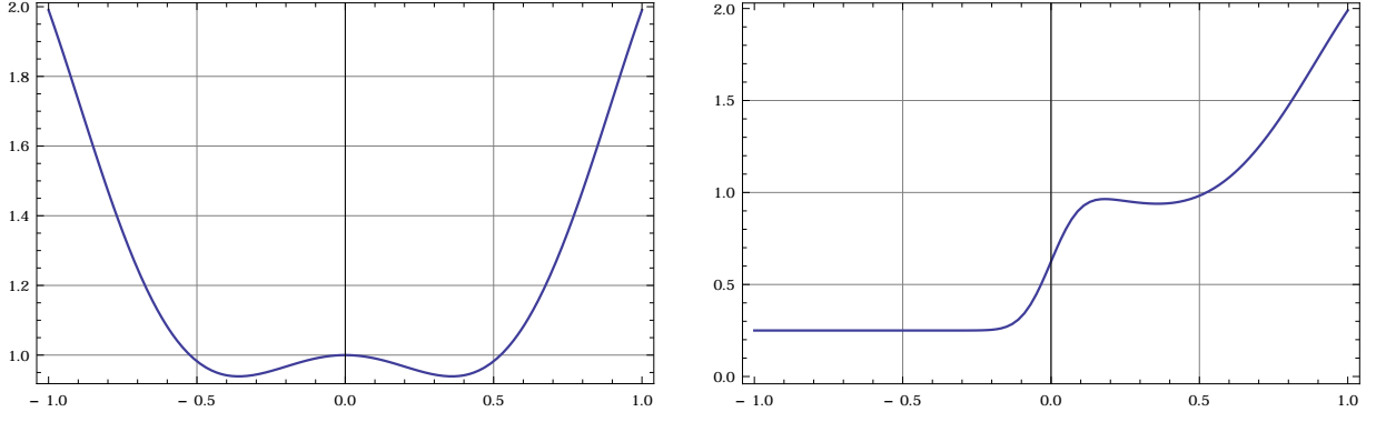
Figure 1: The function q defined by formula (238) in Section 5.1 (left) and the windowed version \tilde{q} of q (right).
