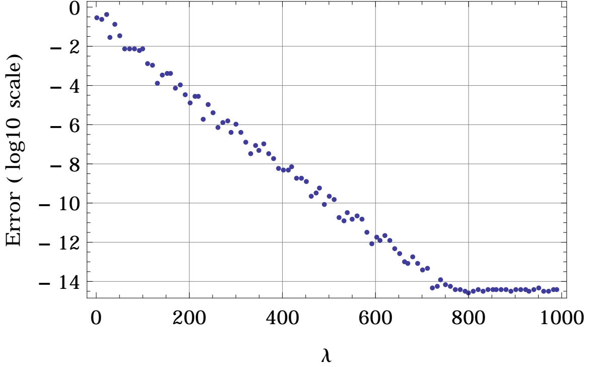
Figure 3: A plot of the base-10 logarithm of the relative difference between phase function obtained by applying the algorithm of this paper to Chebyshev's equation (241) and the well-known nonoscillatory phase function \lambda \arccos(t) for Chebyshev's equation.
