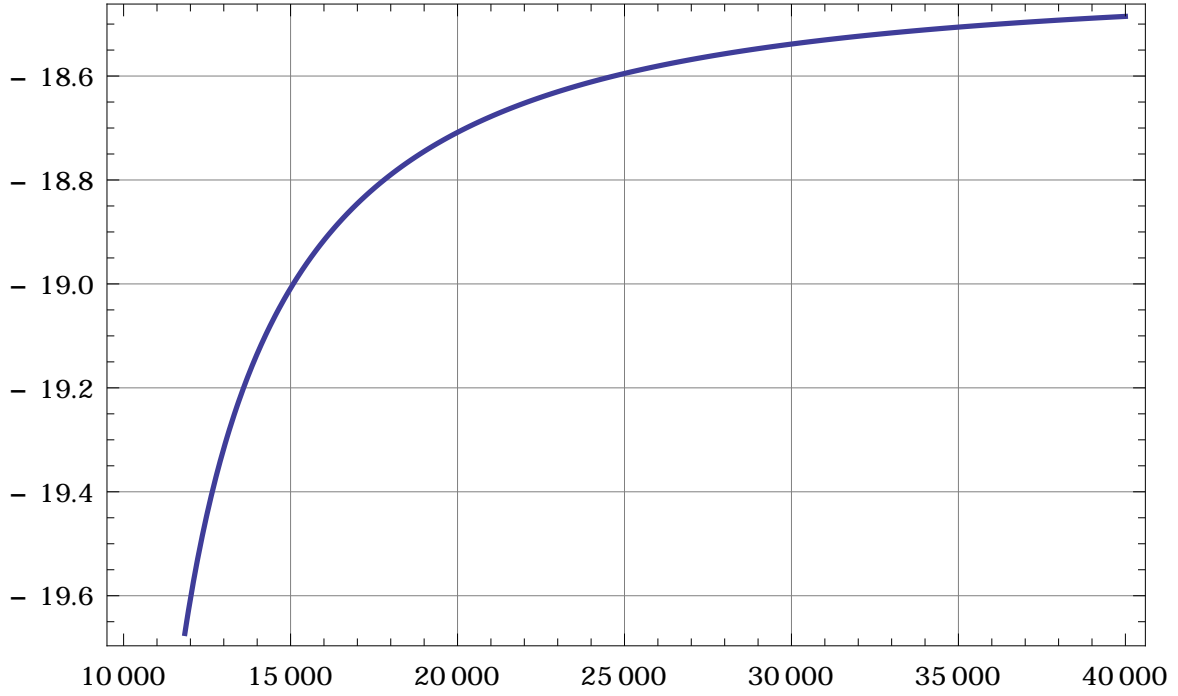
Figure 4: A plot of the nonoscillatory phase function for Bessel's equation (244) when n = 10^4 .
