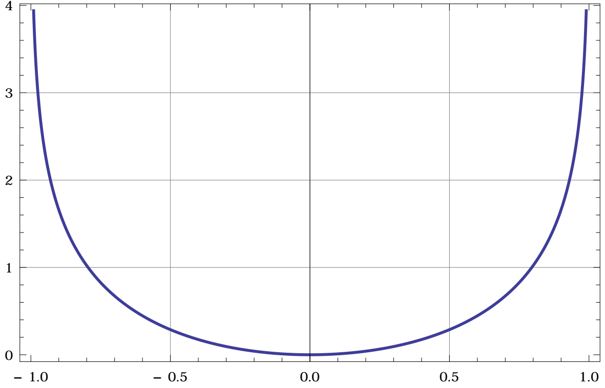
Figure 5: A plot of the nonoscillatory solution of the logarithm form of Kummer's equation associated with Legendre's differential equation (250) when \nu = \pi \cdot 10^5 . This function has singularities at the points \pm 1 and is represented using a graded mesh which becomes dense near them.
