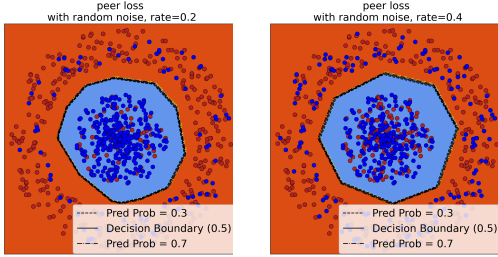
Figure 4. 2D example with peer loss: 20%, 40% random noise.
